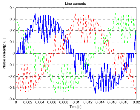
Single bridge MCC
