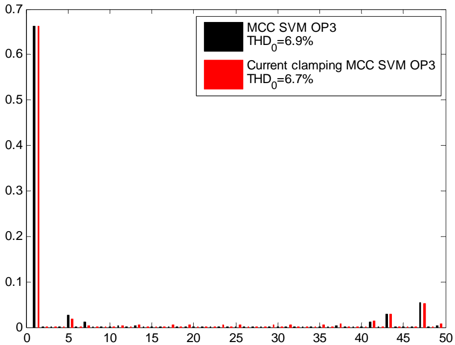
Fig A6 Comparison of harmonic performance between MCC SVM and Current clamping MCC SVM at operating point 3.
