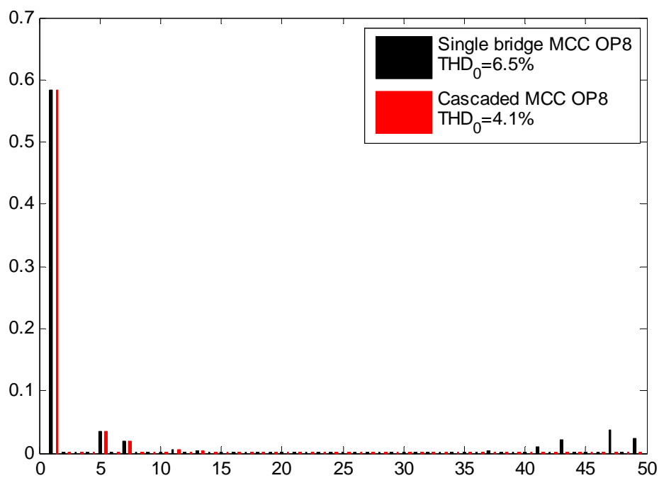
Fig 5.5 Comparison of harmonic performance between single bridge MCC and cascaded MCC at operating point 8, p=48 X_{l-single}=0.2 p.u., X_{l-cascaded}=0.4 p.u.
