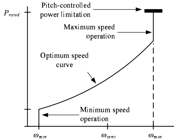
Figure 5.9. Power speed curve.
