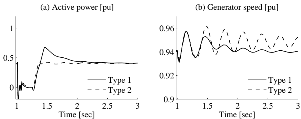
Figure 5.30. Response of two different speed/active power control in DFIG at 0.4 pu power output.
