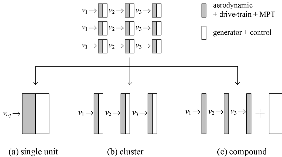
Figure 7.1. Aggregation methods.
