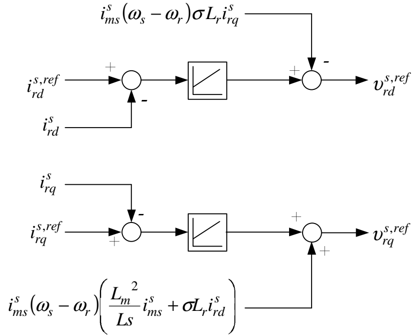
Figure 5.10. Current controller.
