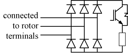
Figure 5.6. Active crowbar.
