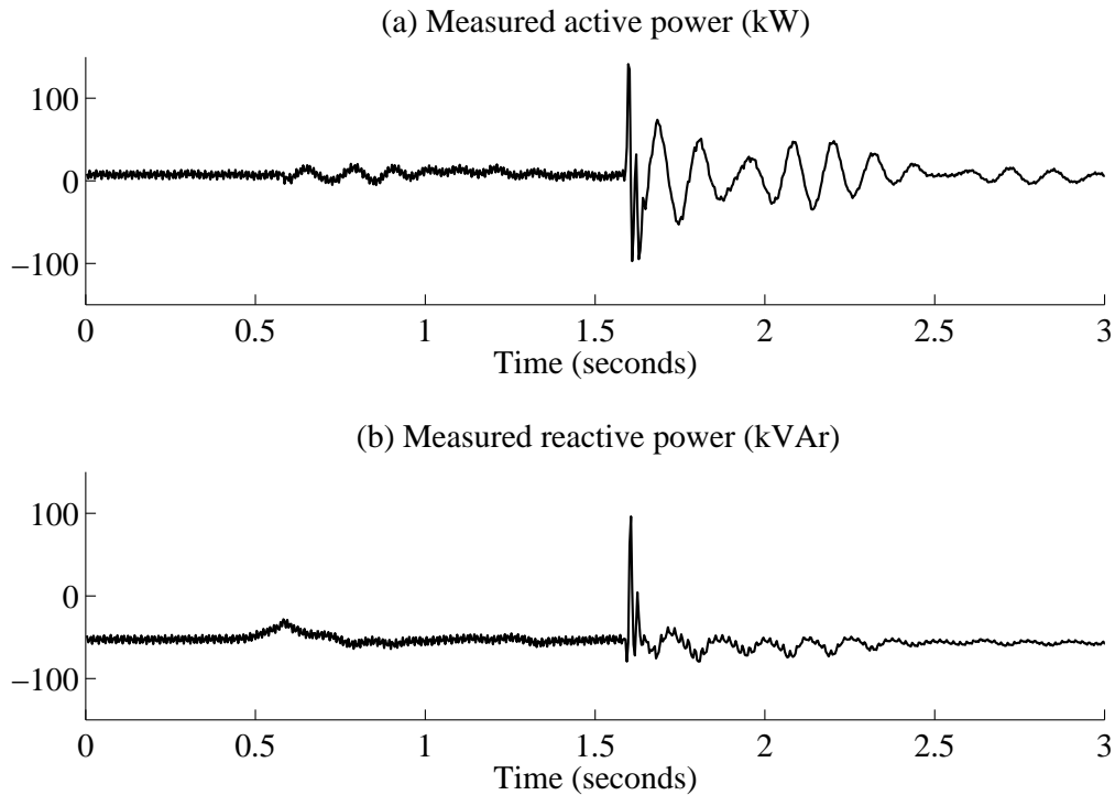
Figure 3.22. Calculated active and reactive power.
