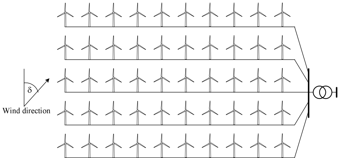
Figure 7.7. Wind farm model layout.
