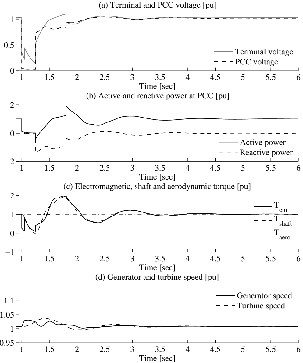
Figure 3.40. Fault ride-through response of fixed-speed wind turbine with SDBR.
