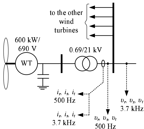
Figure 3.29. Olos single turbine measurement set up.
