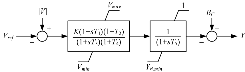
Figure 9.2. Model of SVC in PSS/E (CSVGN1).
