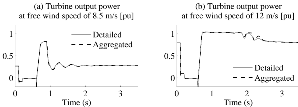
Figure 7.9. Fault response of a wind farm aggregated model consisting of DFIG wind turbine with fast speed control.
