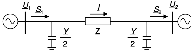
Figure 6.4. One line diagram to illustrate active and reactive power transfer between two generators with a long transmission line.
