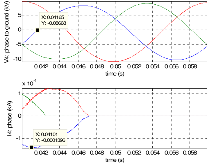
fig. 123. Voltage and current at TP4 when opening at no load
