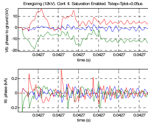
fig. 190. Voltage and Current at tp6 when energizing at no load (12 kV). Saturation modelled
