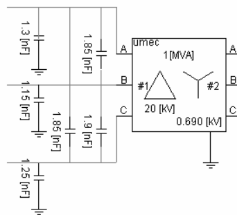
fig. 49. Transformer model for PSCAD
