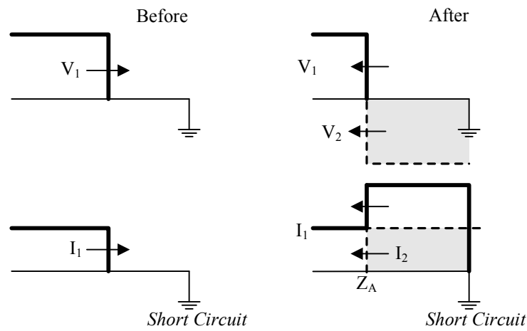
fig. 24. Wave behaviour when encountering a short circuit
