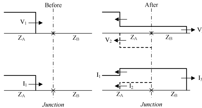
fig. 22. Voltage and Current waves in a line junction
