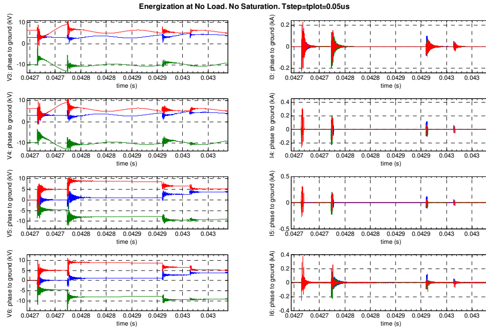
fig. 115. Voltages and Currents in different test points. Energizing at No Load. No Saturation. Tstep=Tplot=0.05μs
