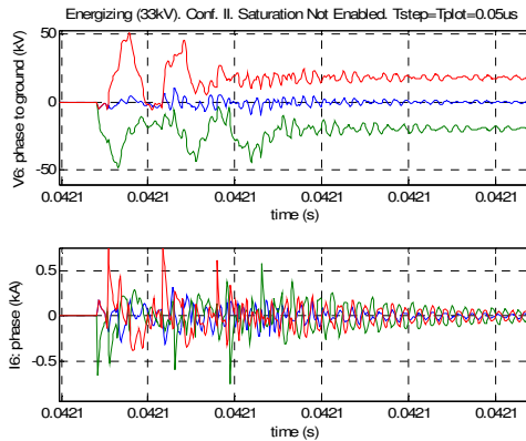
fig. 191. Voltage and Current at tp6 when energizing at no load (33 kV). Saturation not modelled
