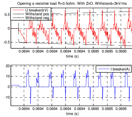
fig. 97. PSCAD: Opening a resistive load ( R=0.5\Omega ) with 11kV ZnO. 10 MS/s
