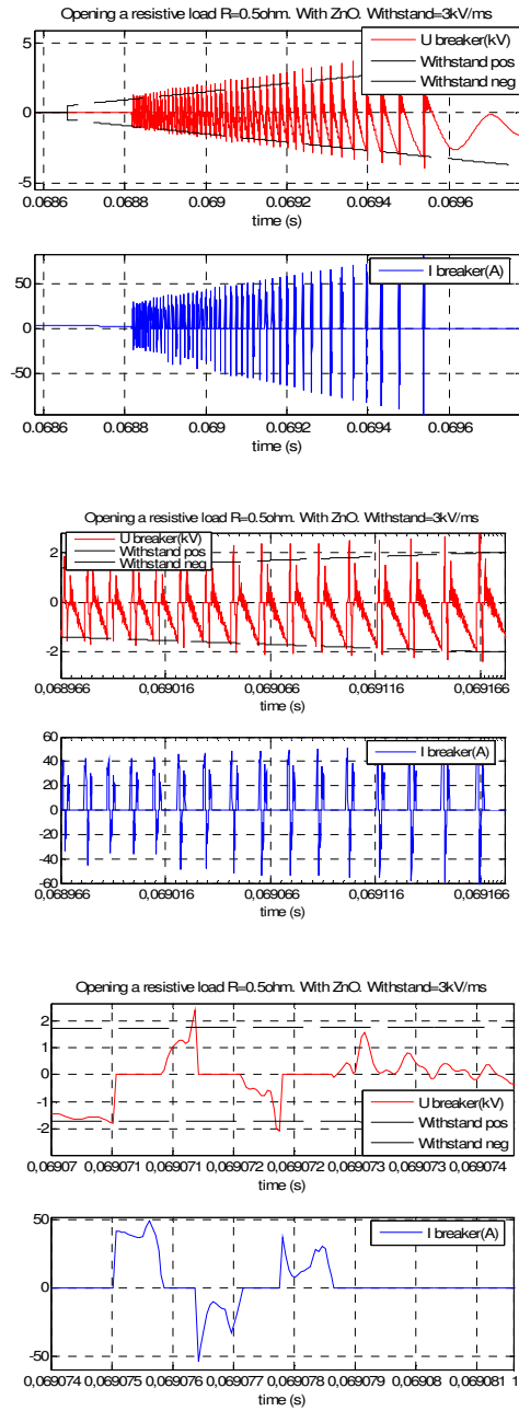
fig. 99. Comparison: Opening a resistive load ( R=0.5\Omega ) with 11kV ZnO. Test: 10Mhz. PSCAD: 0.05\mu s
