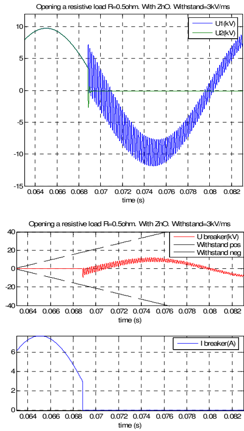
fig. 103. Comparison: Opening a resistive load ( R=0.5\Omega ) with 11kV ZnO. Test: 10Mhz. PSCAD: 0.05\mu\text{s}
