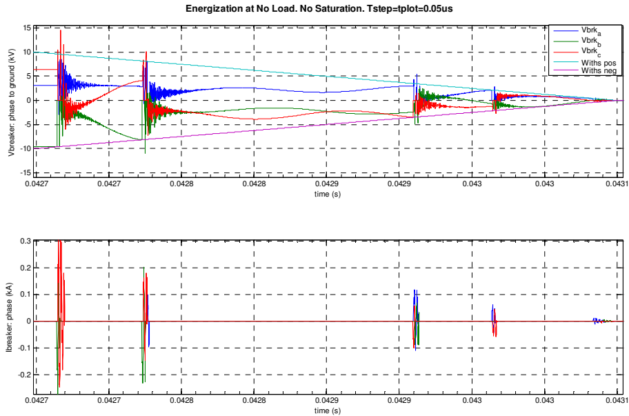
fig. 116. Voltage and Current across the CBs. Energizing at No Load. No Saturation. Tstep=Tplot=0.05μs
