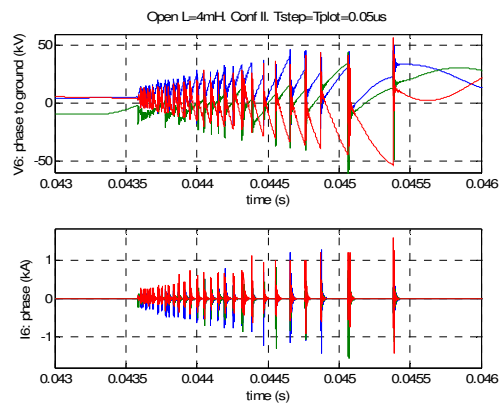
fig. 206. Voltage and Current at tp6 when opening an inductive load (4mH). Saturation Enabled. Configuration II (zoomed)
