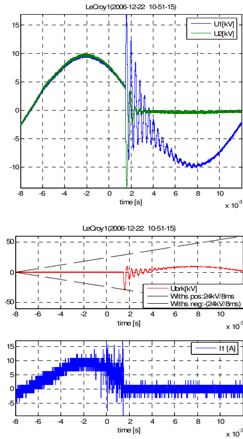
fig. 103. Comparison: Opening a resistive load ( R=0.5\Omega ) with 11kV ZnO. Test: 10Mhz. PSCAD: 0.05\mu\text{s}
