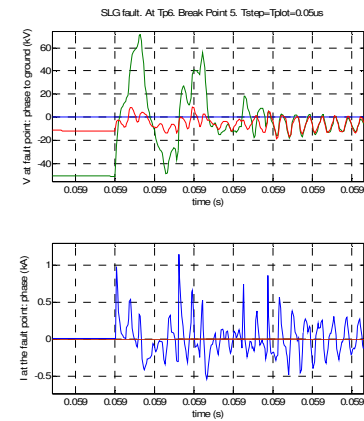
fig. 152. Voltage and Current at fault. Break Point 5
