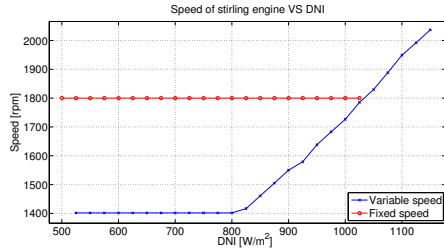
(e) Speed of stirling engine vs DNI
