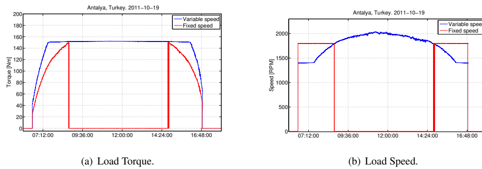
Figure 4.9: Load characteristics for stirling engine based on a to high level of DNI
