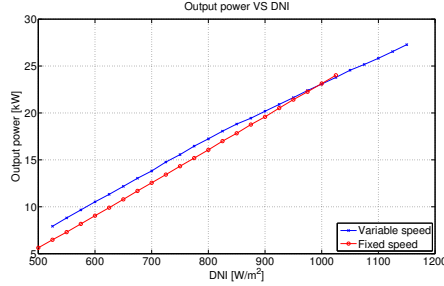
(c) Output power
