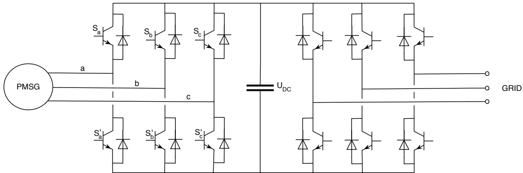
Figure 2.10: Back-to-back PWM conversion schematics
