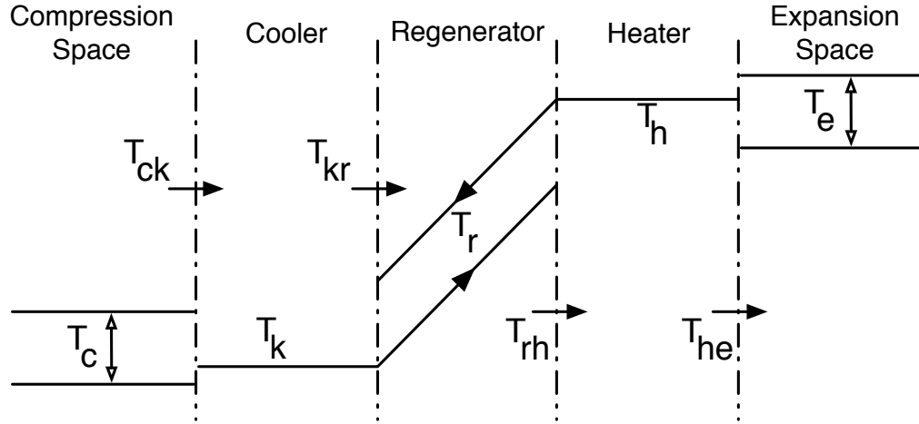
Figure 3.3: Interface temperatures.
