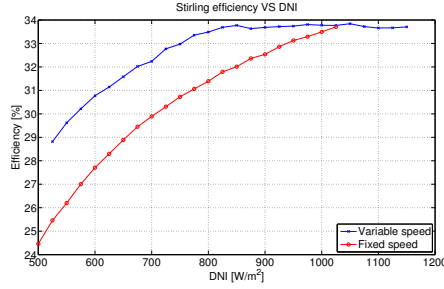
(a) Efficiency of stirling engine.
