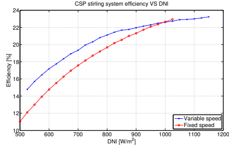
(b) Efficiency of CSP stirling power plant
