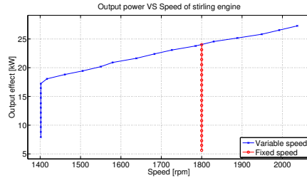
(f) Output power vs Speed of stirling
