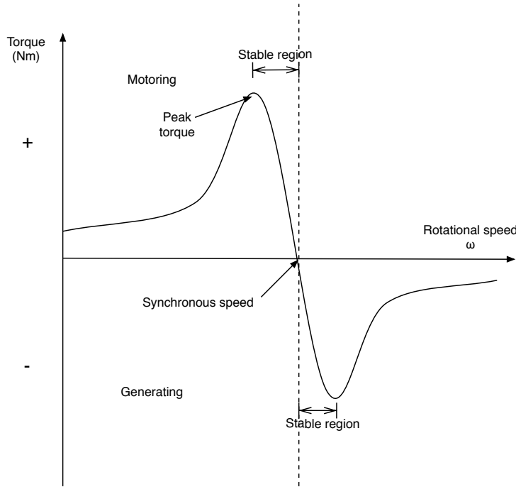
Figure 2.7: Induction machine torque-speed characteristics.
