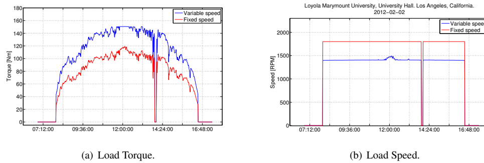
Figure 4.10: Load characteristics for stirling engine based on a to low level of DNI
