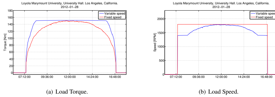
Figure 4.8: Load characteristics for stirling engine based on an optimal level of DNI
