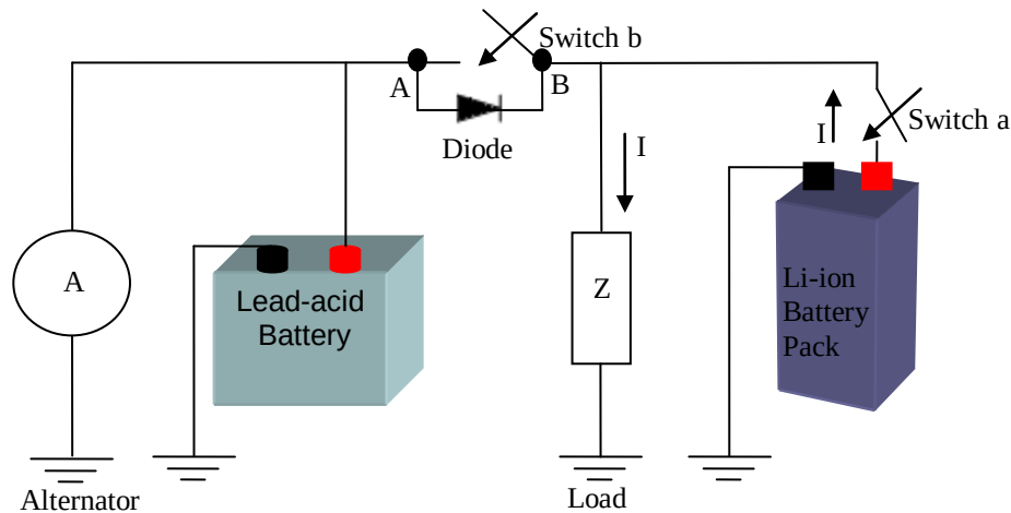
Figure 4.4 Improved battery system solution A in vehicle when the alternator is off
