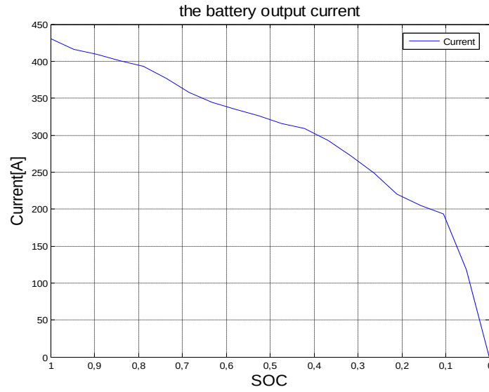
Figure 5.11 The current available for utilization versus SOC for the Li-ion battery pack
