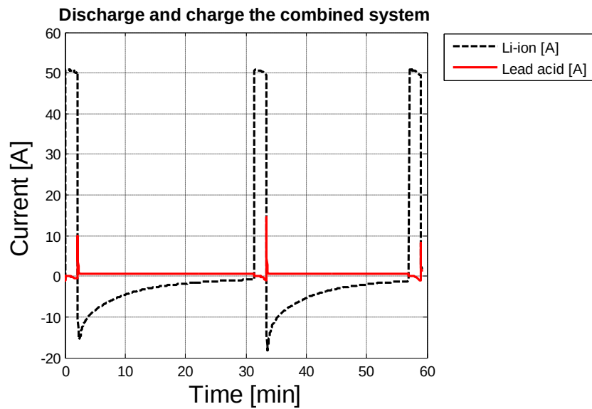
Figure 5.25 Measured currents versus time in the voltage range between 15V and 14.2V
