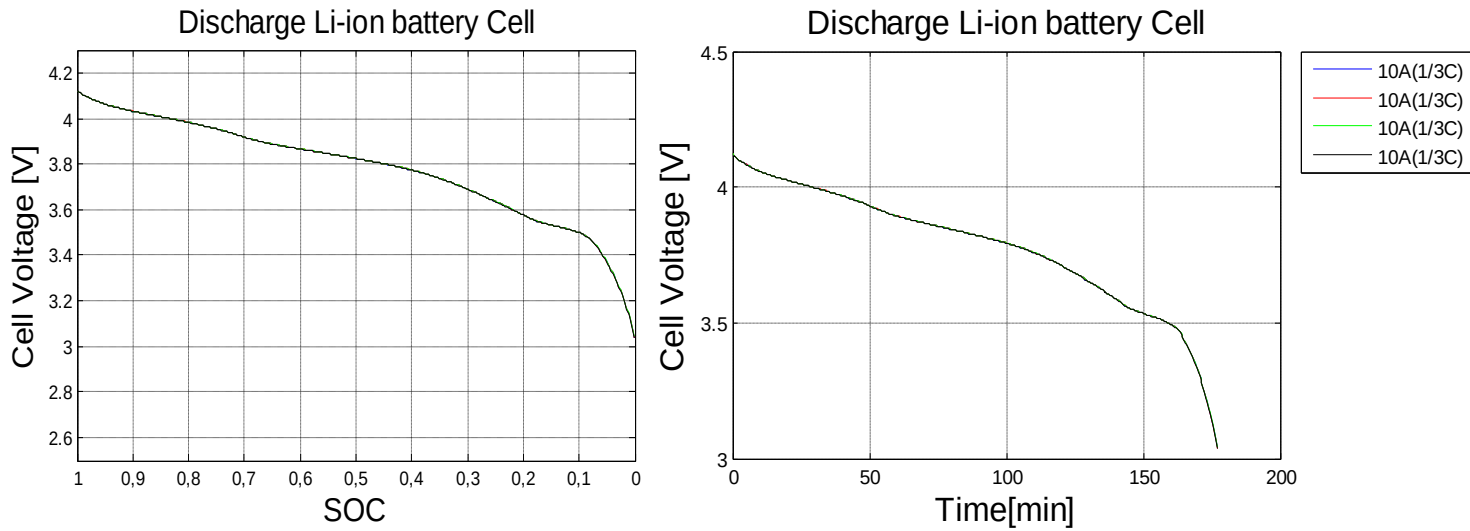
Figure 5.7 Cell Voltage vs Time for each cell in the battery pack during discharging time
