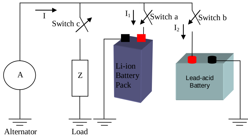
Figure 5.13 The model during charging of the batteries
