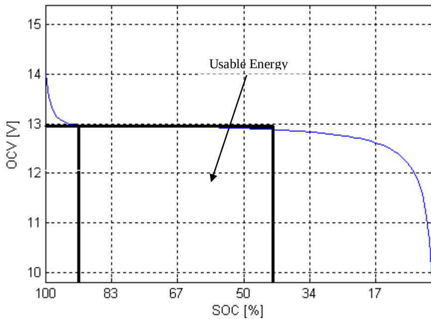
Figure 7.1 OCV versus SOC for the future battery type.
