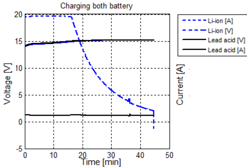
Figure 5.15 The current and voltage over both battery packs during charge
