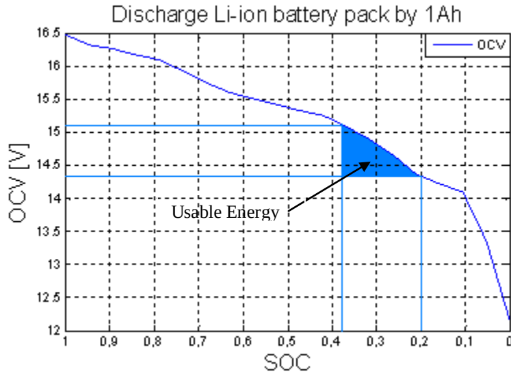
Figure 5.14 Discharge of the Li-ion battery pack with respect to OCV vs SOC, with the total capacity 26.67Ah
