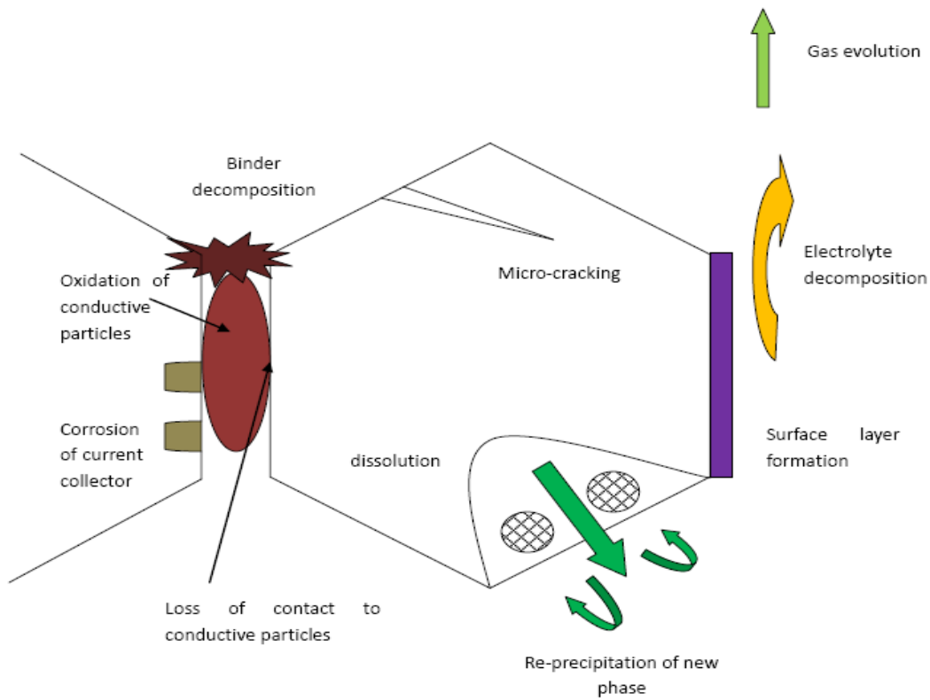
Figure 2.6 Changes at the cathode
