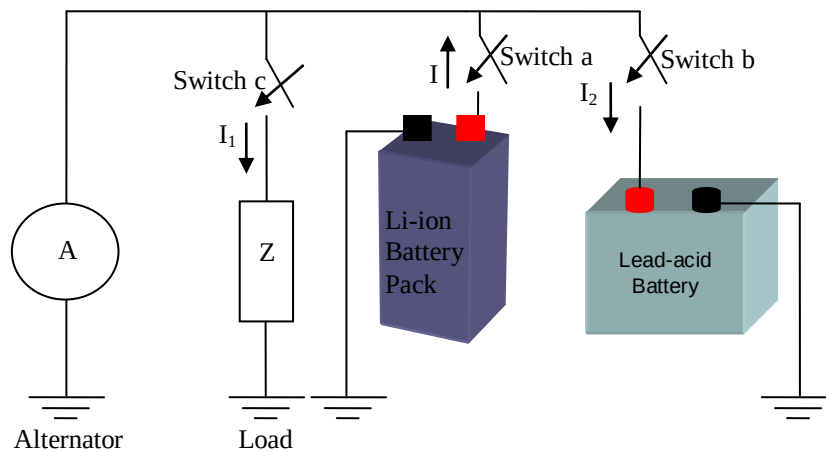
Figure 5.17 The first model during discharge of the batteries
