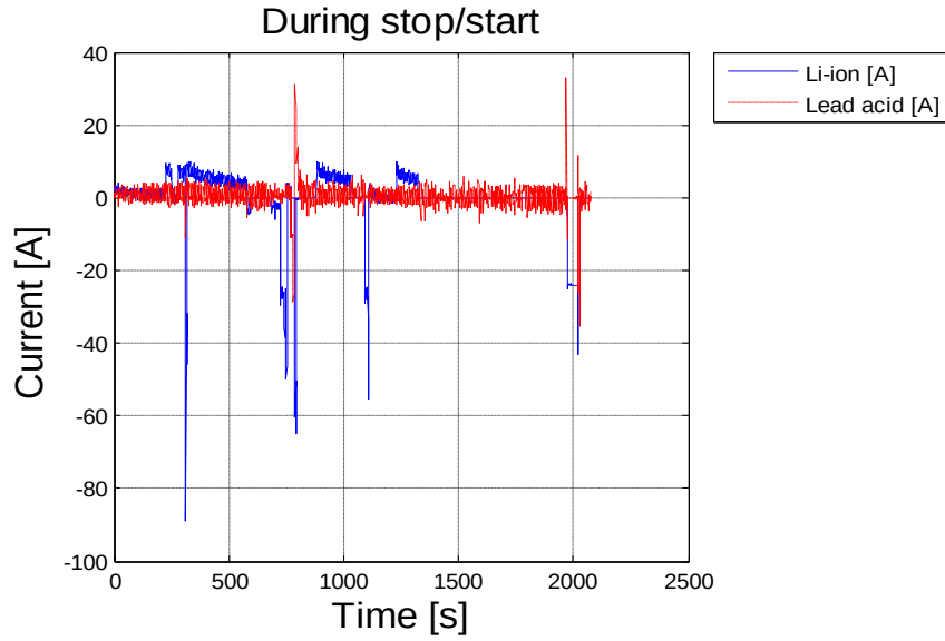
Figure 5.33 Measured currents versus time from repeated tests in the vehicle
