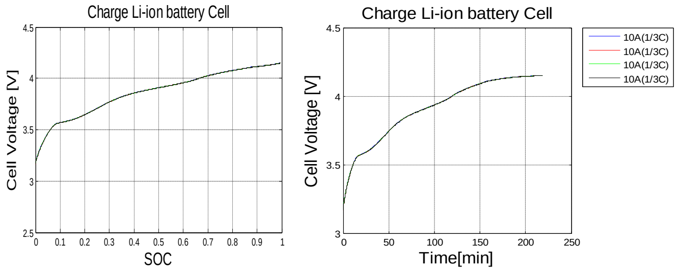
Figure 5.6 Cell Voltage vs SOC and Time for each cell in the battery pack during charging time
