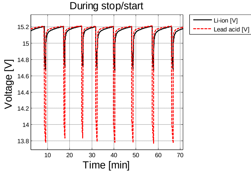
Figure 5.22 The terminal voltage over both battery packs during stop/start time, CV
