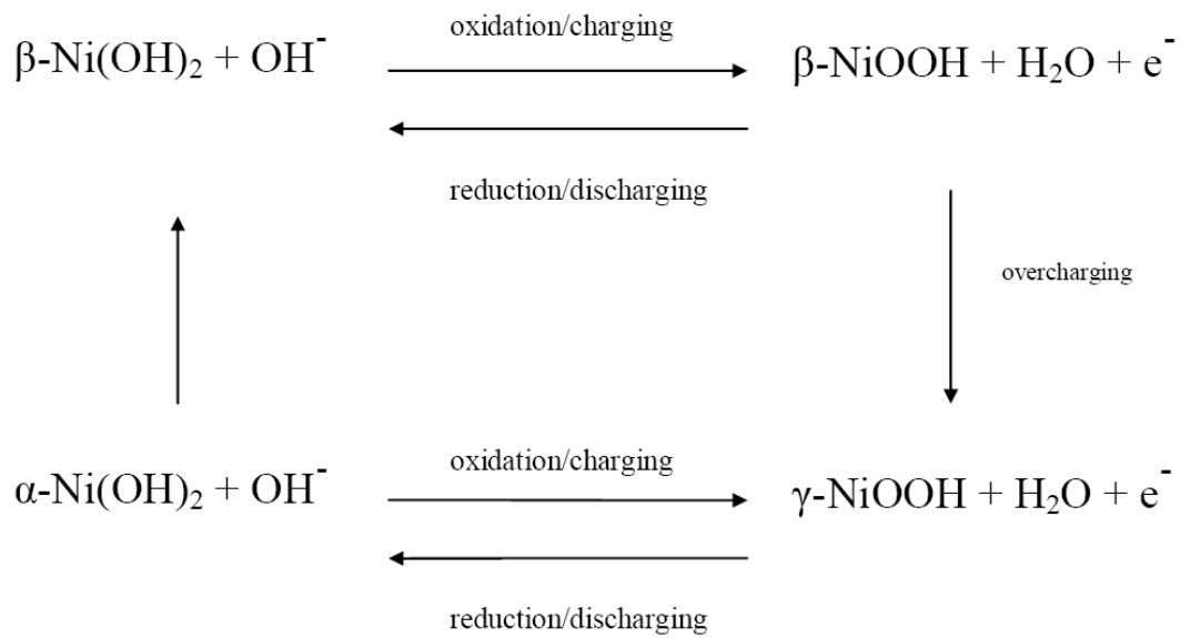
Figure 2.9 Phase transformation inside nickel-based batteries
