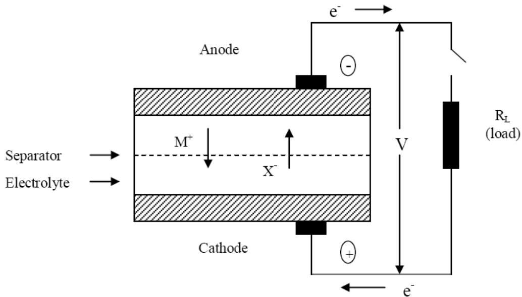
Figure 2.1 Sketch of components of a cell with current flows during discharge
