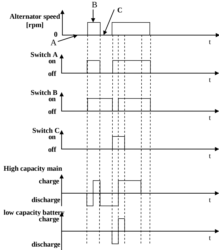
Figure 1.3 Charge and discharge procedure in start-stop application
