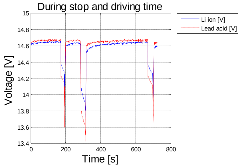
Figure 5.31 Measured voltages versus time from the tests in the vehicle
