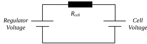
Figure 3.1 Equivalent circuit model for the CC-CV method of charging a Li-ion cell
