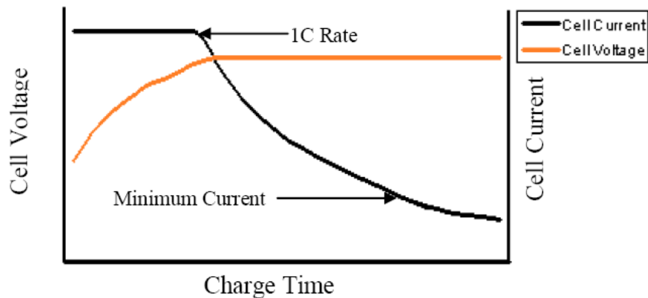
Figure 3.6 The Li-ion charging characteristics
