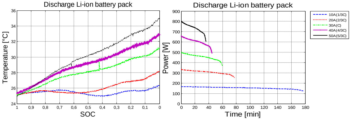
Figure 5.2 Measured Temperature vs SOC (left) and Power vs Time (right) at different discharges current
