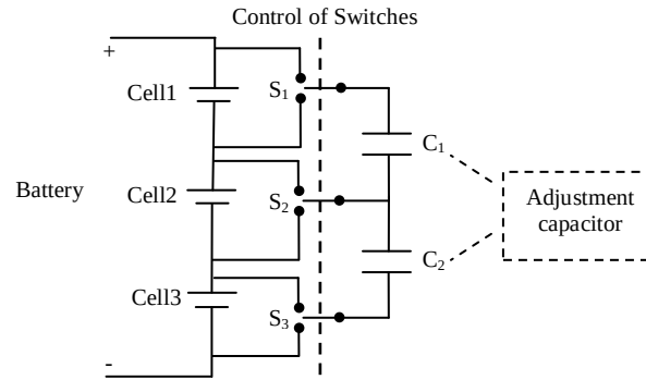
Figure 3.5 Switched capacitor equalization method
