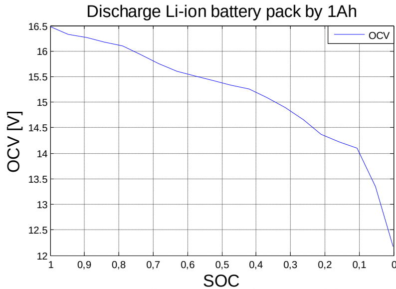
Figure 5.10 Discharging Li-ion battery pack by 1/30C, OCV vs SOC.
