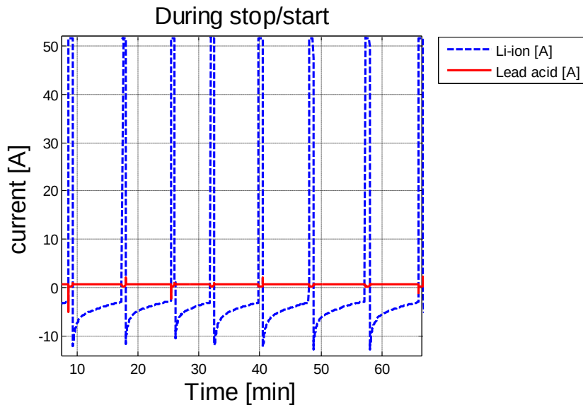
Figure 5.21 The in/out put current through both battery packs during stop/start time, CV (negative values mean charging current)
