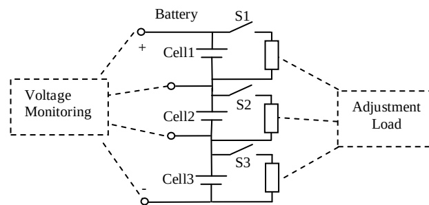
Figure 3.3 Resistive equalization method
