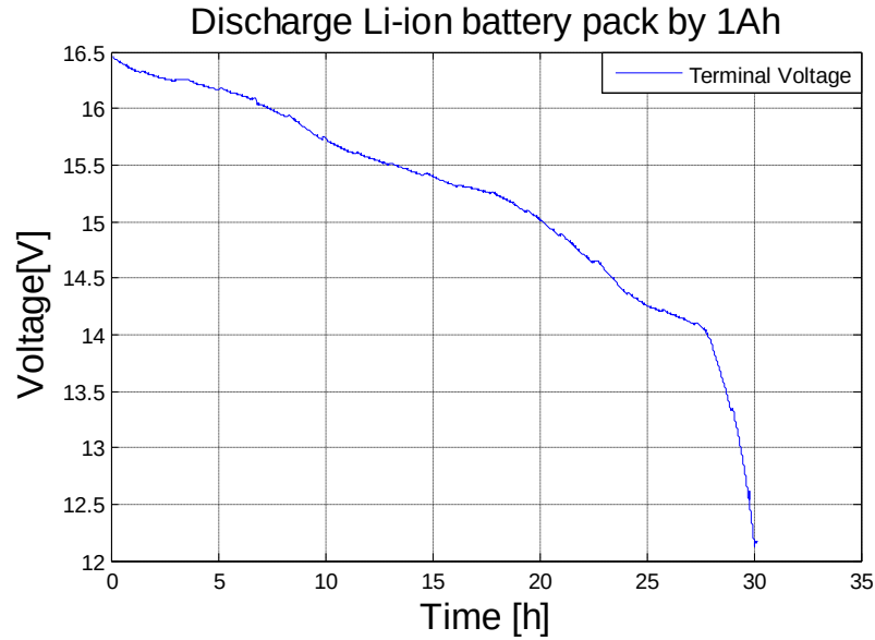
Figure 5.9 Terminal Voltage vs Time by discharging at 1/30C rate
