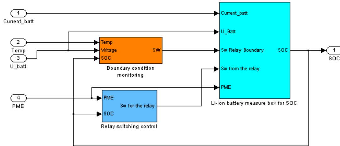
Appendix A figure1. The main Simulink model
