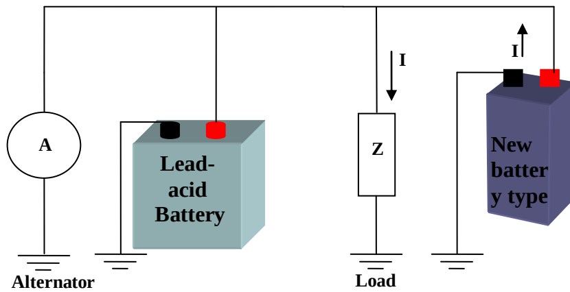
Figure 1.4 Improvement of the start-stop application in vehicles
