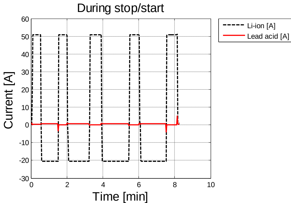
Figure 5.23 The in/output current through both battery packs during charge and discharge time, CC
