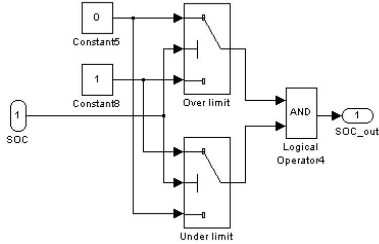
Appendix A figure11. The SOC control block
