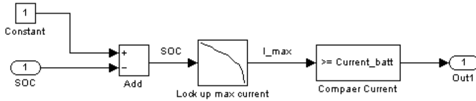
Appendix A figure12. The max current limit block
