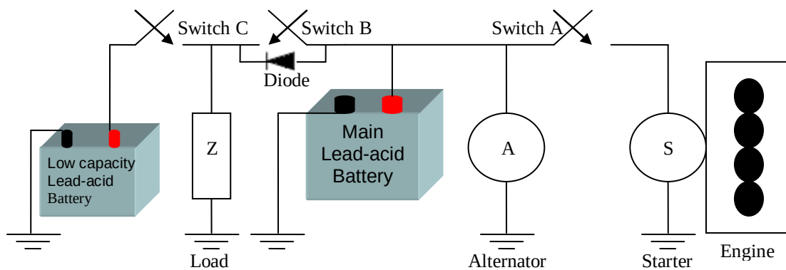
Figure 1.2 Dual battery systems in the start-stop application
