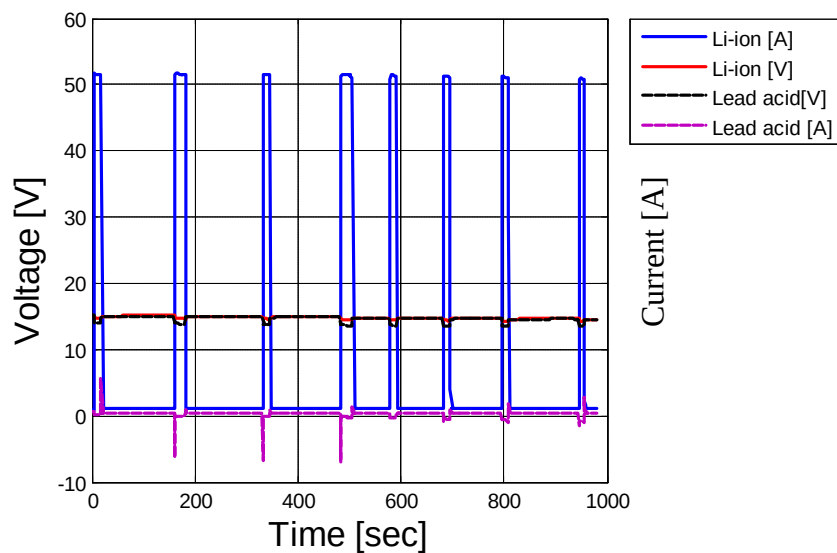
Figure 5.18 Measured voltage and current versus time during the stops
