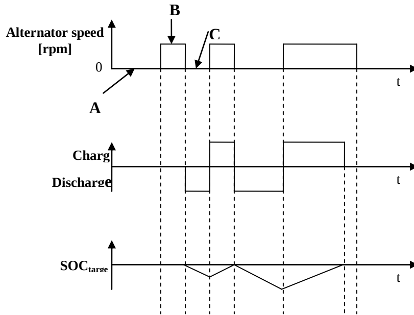
Figure 4.9 The function of the engine to be on or off affects the charge and discharge of the Li-ion battery pack
