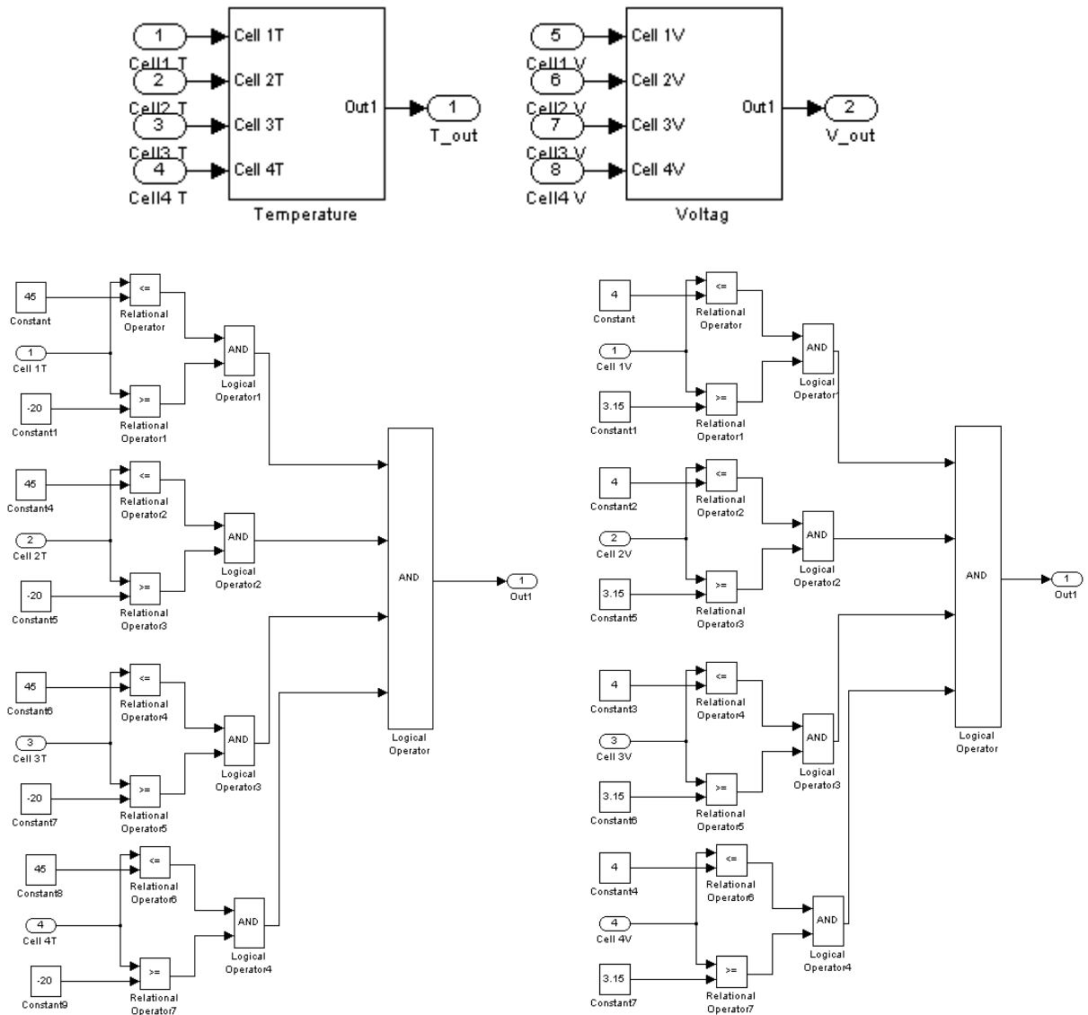
Appendix A figure10. The temperature & voltage conditions block
