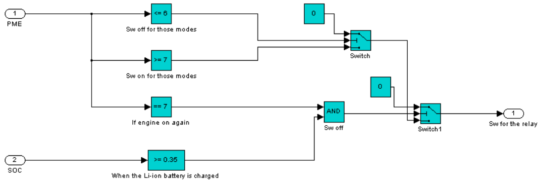
Appendix A figure8. The relay A switching control block
