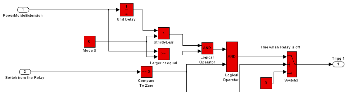
Appendix A figure6. Block for determining trigger A
