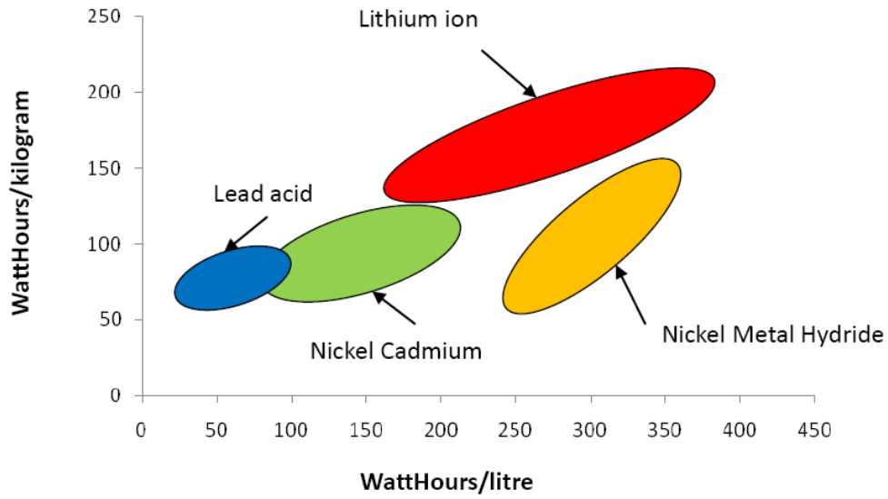
Figure 2.7 Comparison of energy density for different types of batteries
