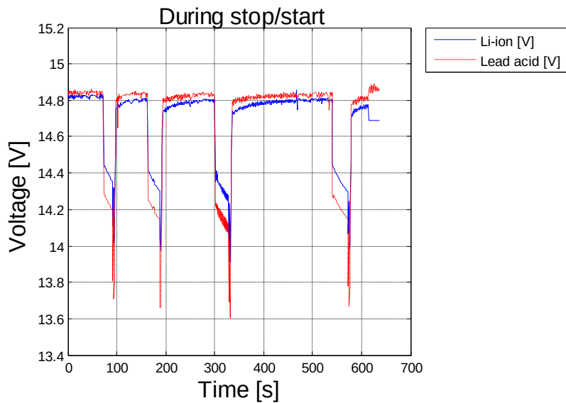
Figure 5.30 The voltage versus time for both batteries pack in the vehicle
