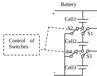
Figure 3.2 Parallel charging method
