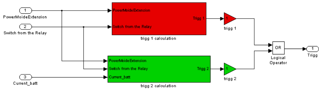
Appendix A figure5. Block for calculating trigger
