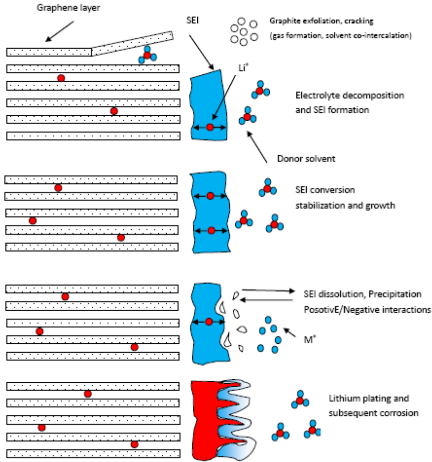
Figure 2.5 Change at the anode/electrolyte interface
