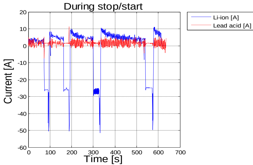
Figure 5.29 The current flow for both battery packs in the vehicle
