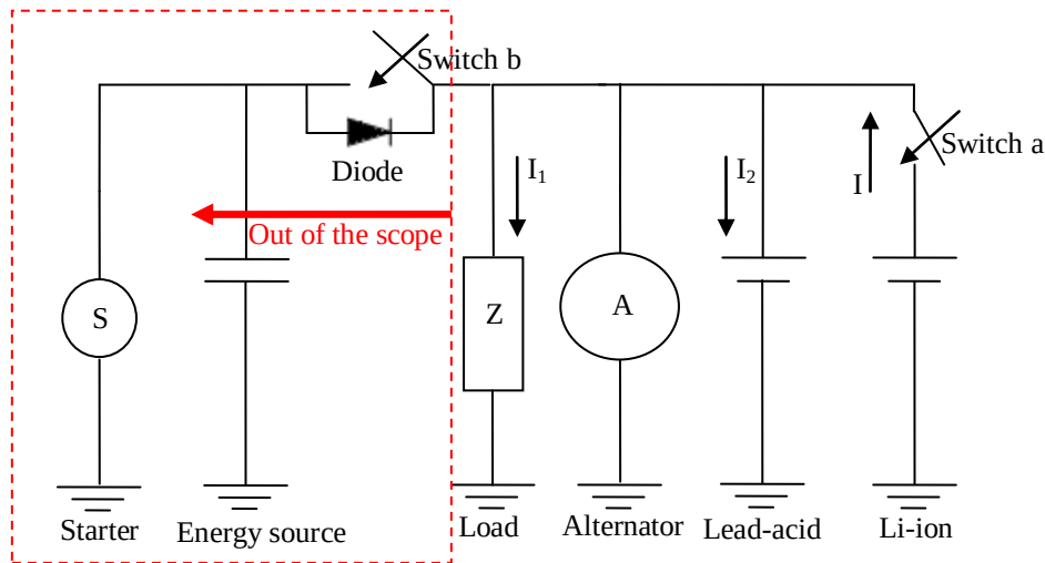
Figure 4.6 Connection system of both battery types in the vehicle
