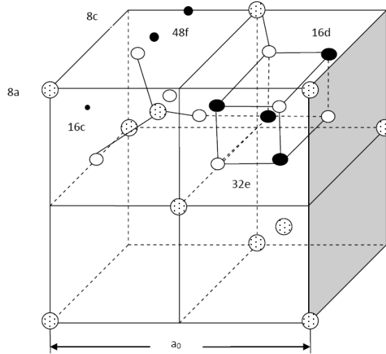
Figure 2.12 Two quadrants of cubic spinel structures
