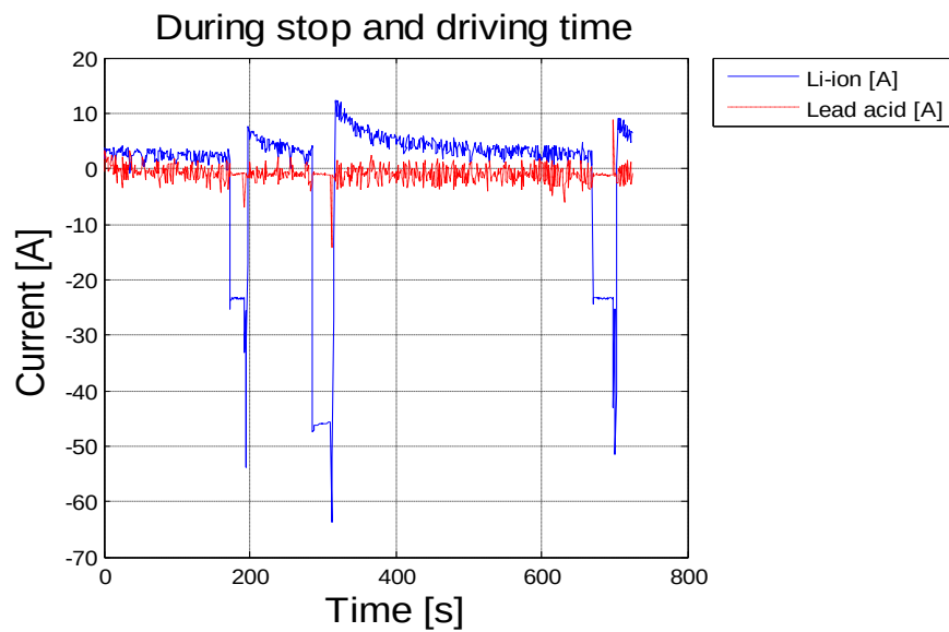
Figure 5.32 Measured currents versus time from the tests in the vehicle
