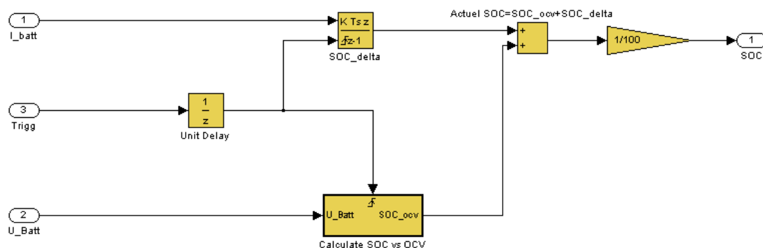
Appendix A figure3. The Li-ion battery measure box for the SOC block
