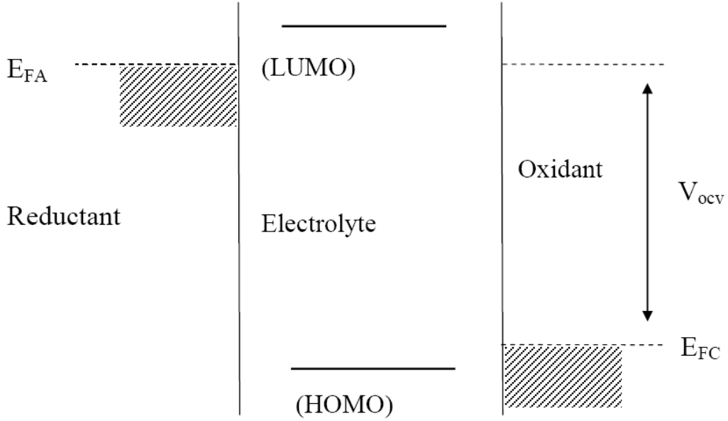
Figure 2.8 The role of Fermi energy for the two electrodes and LUMO and HOMO for the electrolyte to achieve a stable battery
