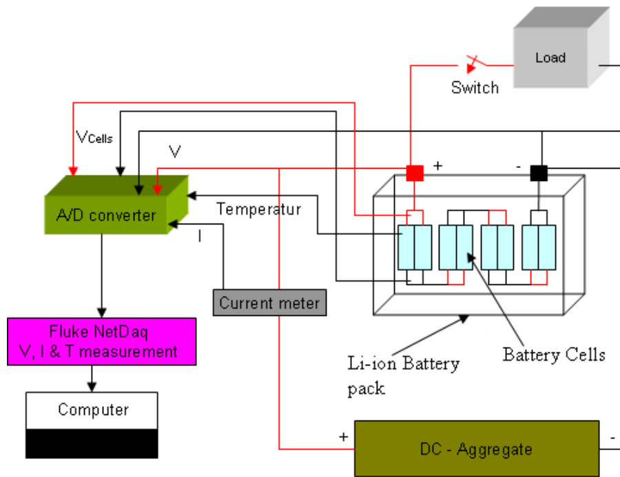
Figure 4.1 Sketching charge/discharge system.
