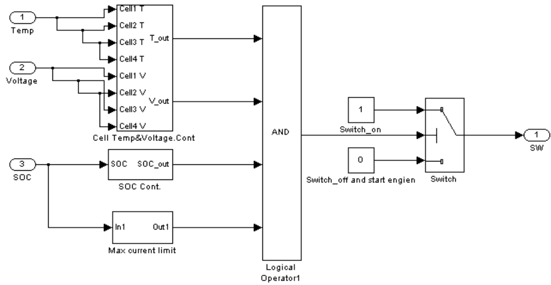
Appendix A figure9. The boundary condition for the monitoring block
