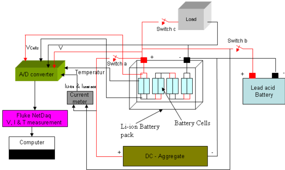
Figure 5.12 The connected model at the lab bench
