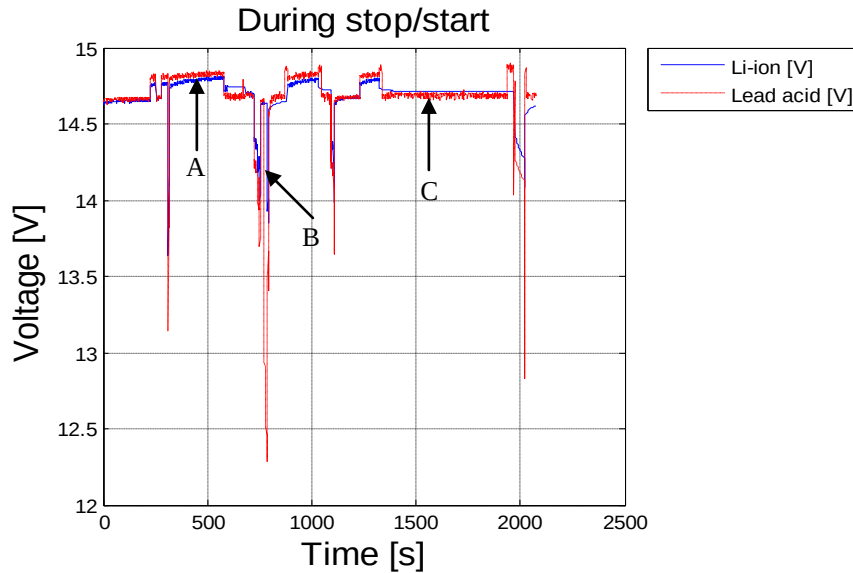
Figure 5.34 Measured voltage versus time from repeated tests in the vehicle
