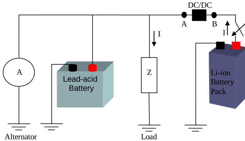
Figure 4.5 Improved battery system solution A in vehicle when the alternator is off
