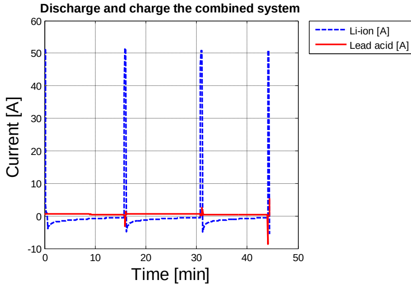
Figure 5.27 Measured currents versus time in the voltage range between 15V and 14.6V
