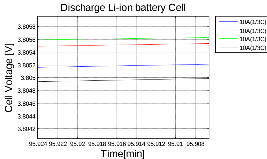
Figure 5.8 Enlarged graphs of Figure 5.7
