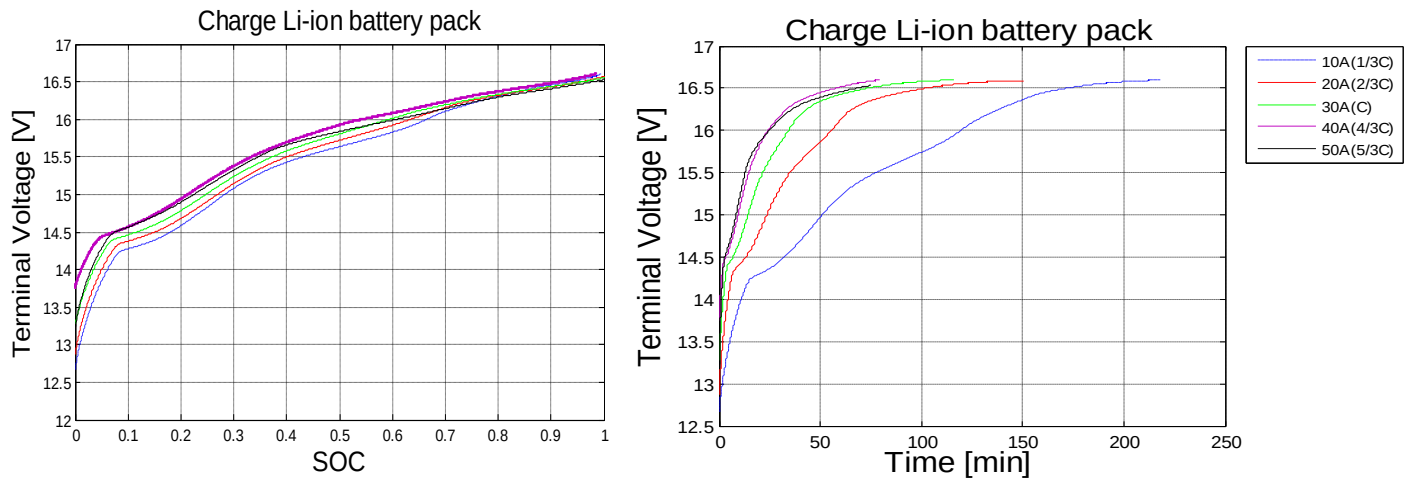
Figure 5.3 Measured Terminal Voltage vs SOC (left) and Terminal Voltage vs Time (right) at different charges current
