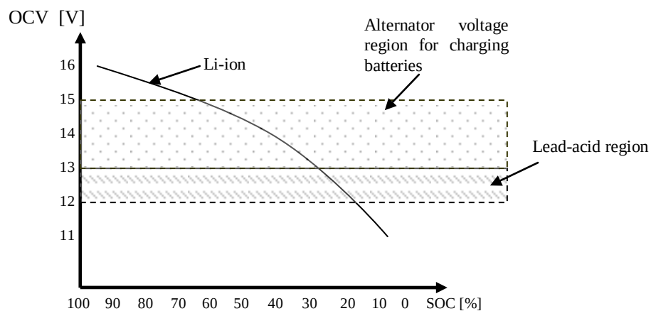
Figure 4.3 A comparison of OCV of Li-ion battery and lead-acid battery
