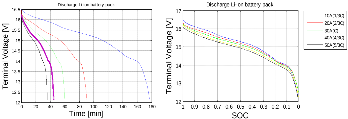
Figure 5.1 Measured Terminal Voltage vs Time (left) and Terminal Voltage vs SOC (right) at different discharging currents
