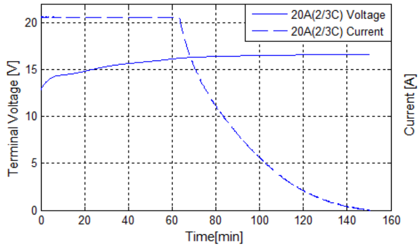
Figure 5.5 Charging characteristics for lithium ion battery in the experiments
