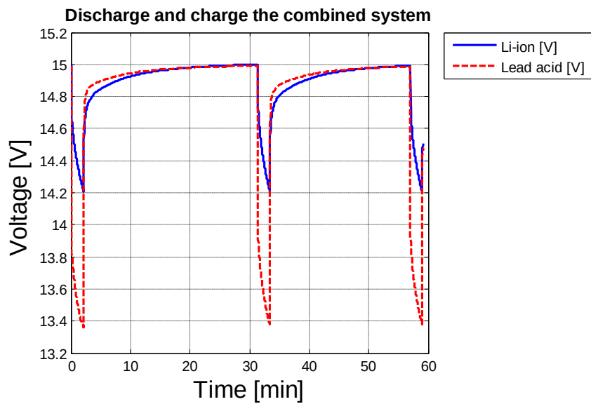
Figure 5.26 Measured voltages versus time in the voltage range between 15V and 14.2V
