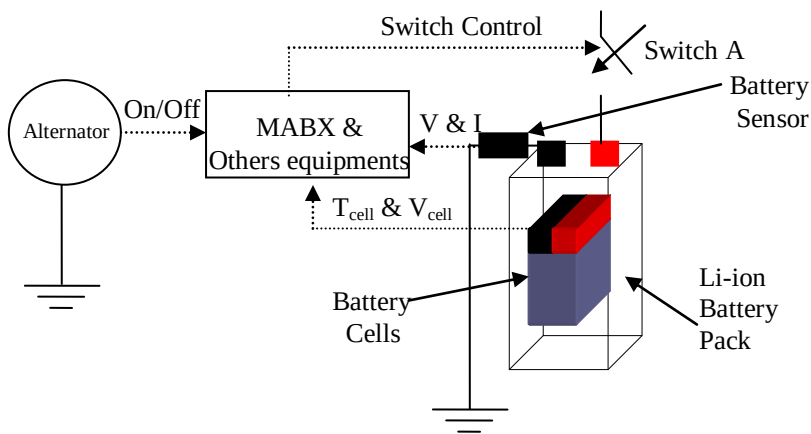
Figure 4.8 The controller system for the Li-ion battery pack
