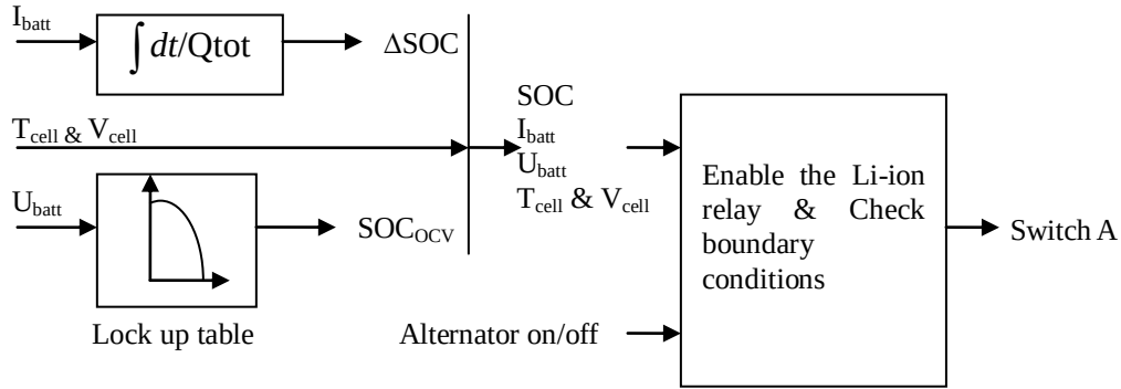
Figure 4.7 Charge and discharge battery model chart of Li-ion battery pack
