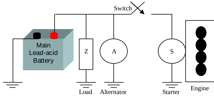
Figure 1.1 An overview of the battery behavior in a conventional vehicle
