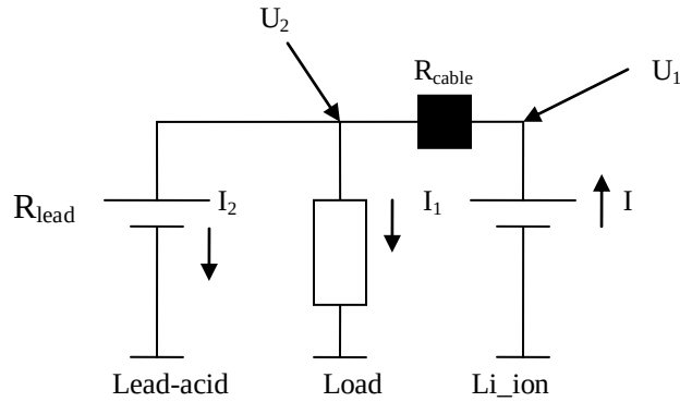
Figure 5.20 The combined system during discharging
