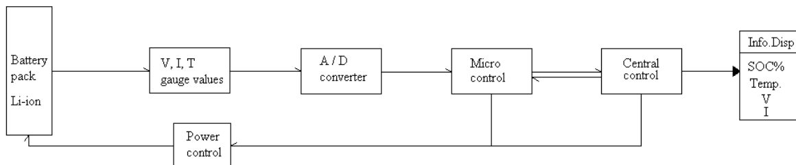
Figure 2.14 Scheme of the controller system for Li-ion battery packs
