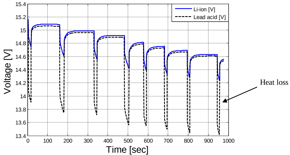
Figure 5.19 The terminal voltages over both batteries
