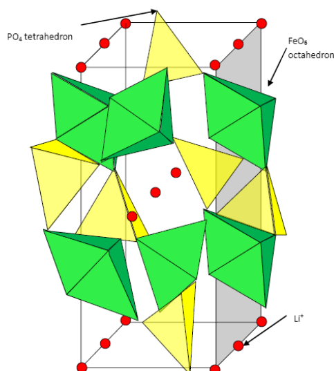
Figure 2.13 Structure of \text{LiFePO}_4
