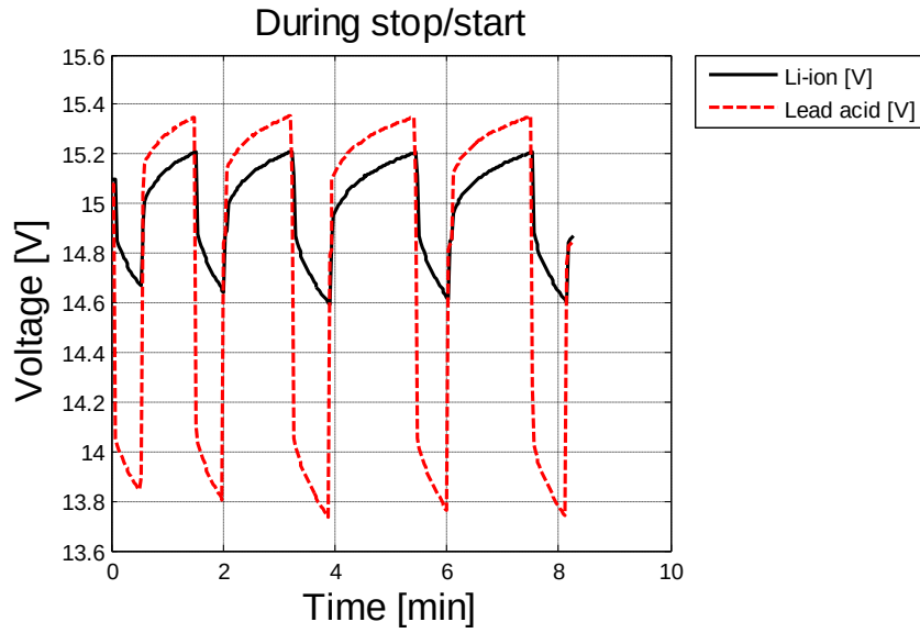
Figure 5.24 The thermal voltage over both battery packs during charge and discharge time, CC
