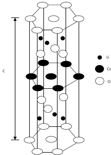
Figure 2.11 Structure of \text{LiCoO}_2
