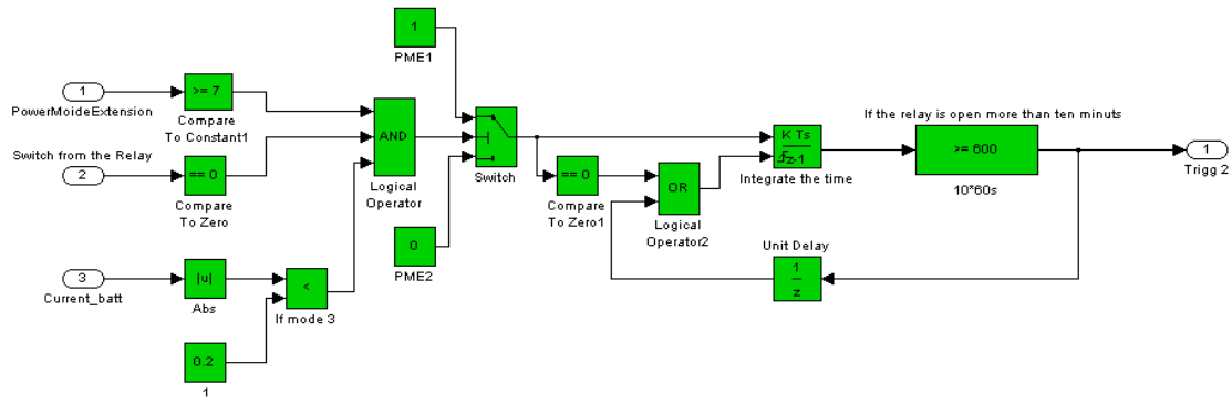
Appendix A figure7. Block for calculating trigger 2
