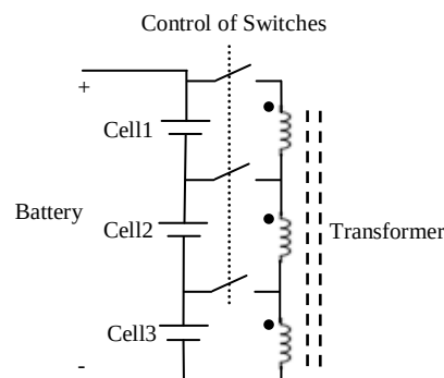
Figure 3.4 Transformer equalization method
