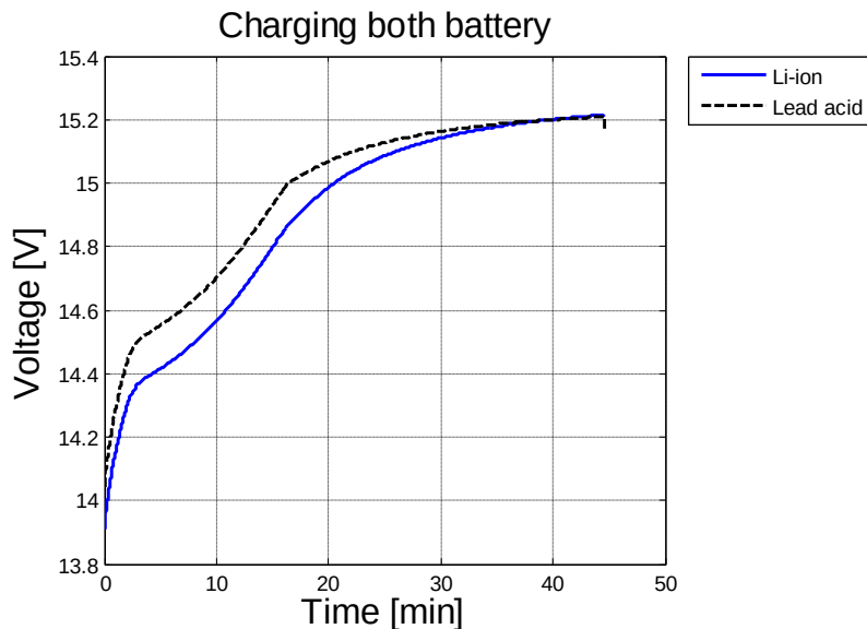
Figure 5.16 The voltage versus time during charging of the combined system
