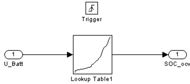
Appendix A figure4. The SOCocv calculation block
