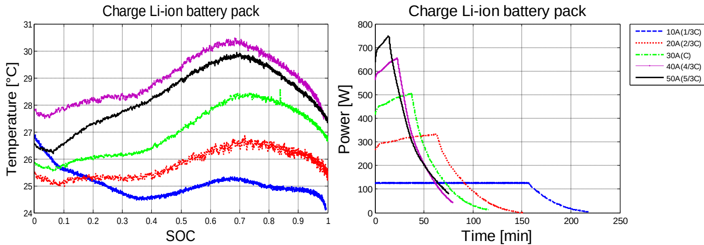
Figure 5.4 Measured Temperature vs SOC (left) and Power vs Time (right) at different charges currents
