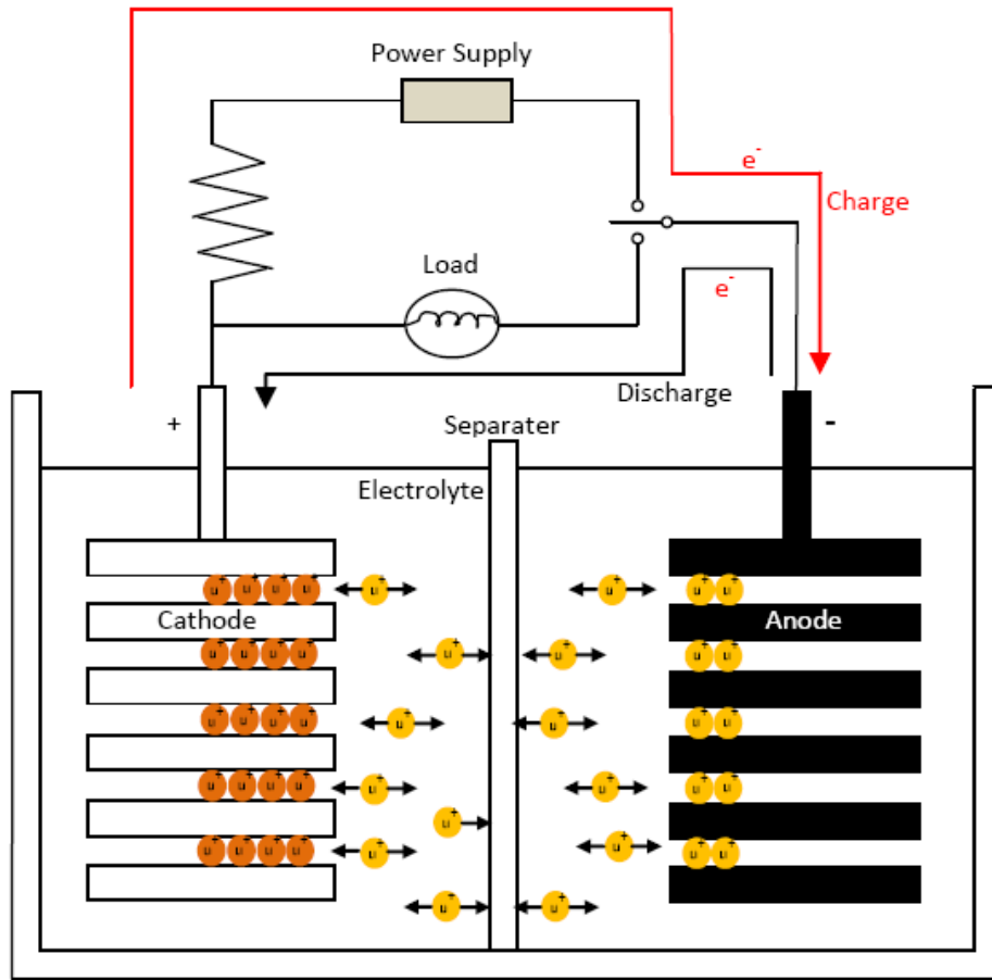
Figure 2.4 The principle of lithium-ion battery
