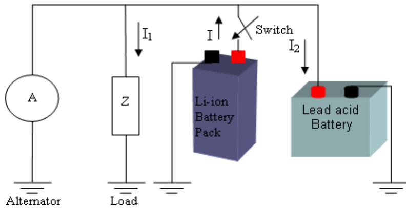
Figure 4.2 The original battery system solution in the vehicle when the alternator is off
