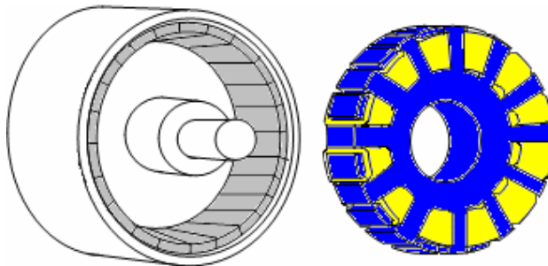
Figure 29. Stator and rotor of an outer rotor PM motor [NTNU].
