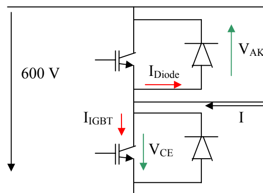
Figure 8. Test circuit.
