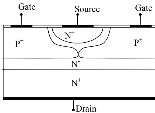
Figure 52. SIT.
