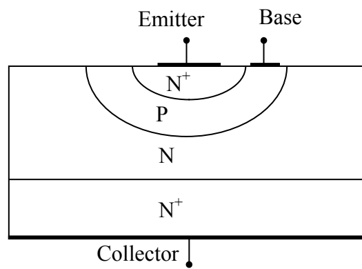
Figure 53. BJT.
