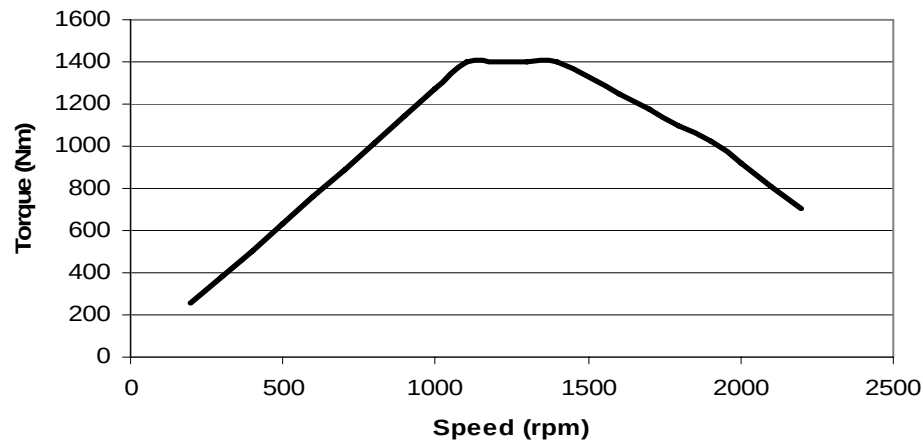
Figure 31. Speed vs. torque for the diesel engine.
