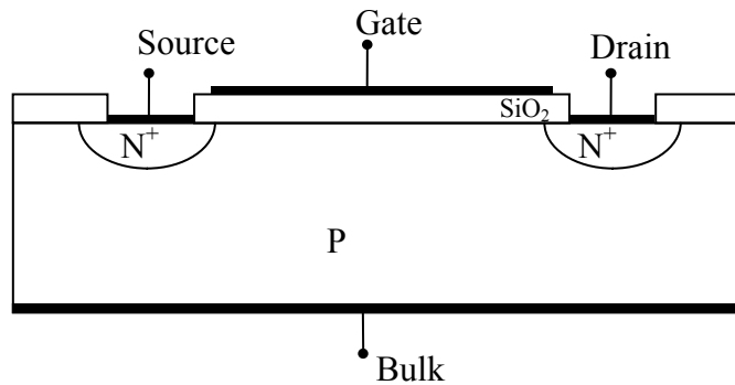
Figure 46. Basic MOSFET.
