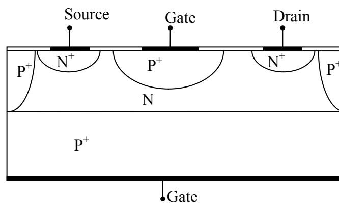
Figure 50. JFET.
