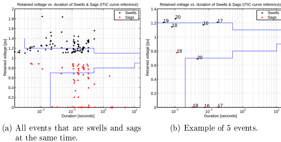
Figure 5.5: Retained voltage vs. duration for events that are swells and sags.
