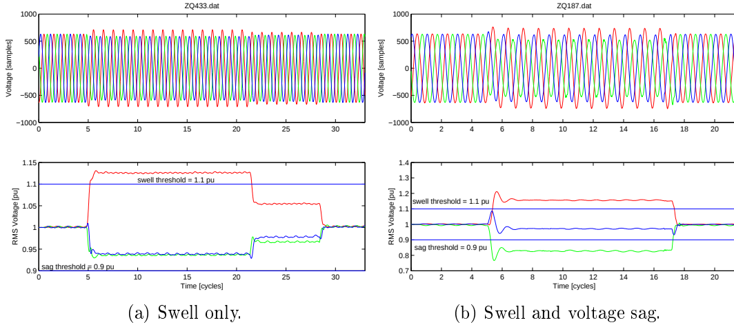
Figure 3.7: Swells.
