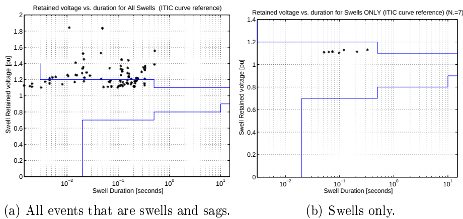
Figure 5.6: Retained voltage vs. duration for events classified as swells.
