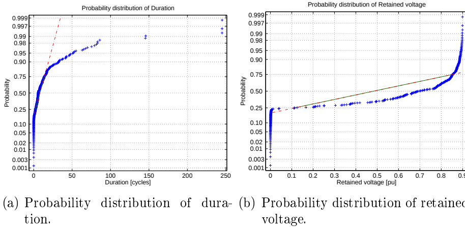
Figure 3.15: Probability distribution of duration and retained voltage for all sags.
