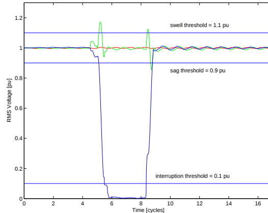
Figure 1.1: Example of voltage sag, interruption and swell in one event
