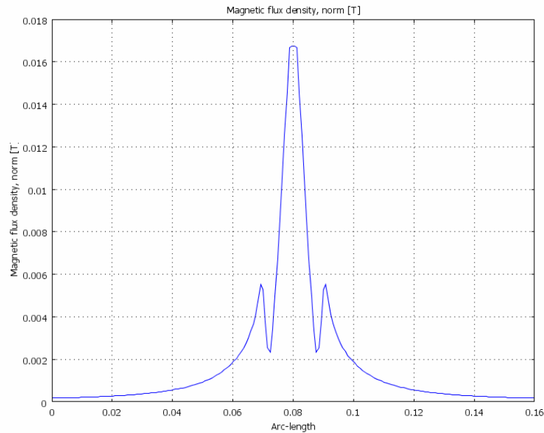
Figure 6.24 - Vertical cross-section plot of the magnetic flux density of two cables with no distance between them and next to a magnetic girder.
