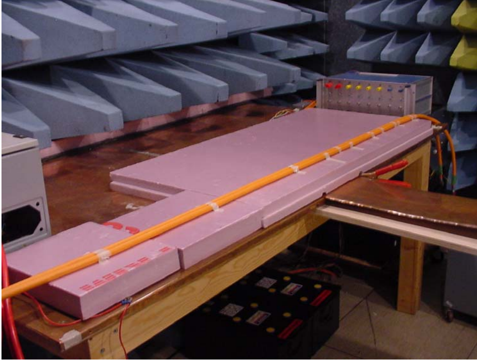
Figure 3 - The shielded cables placed with no distance between them 5 cm from the grounded plane.
