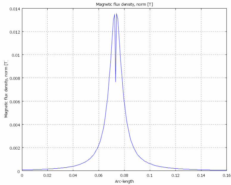
Figure 6.41 - Horizontal cross-section plot of the magnetic flux density for a cable with two conductors with a common shield and a distance of 0.5 m to the magnetic girder.
