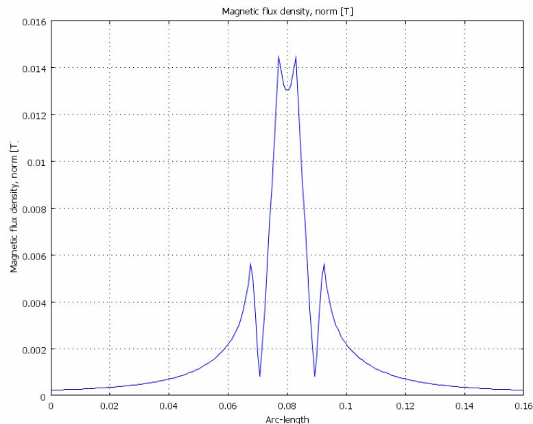
Figure 6.36 - Vertical cross-section plot of the magnetic flux density of two shielded cables with no distance between them and placed next to a magnetic girder.
