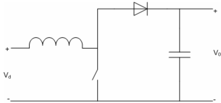
Figure 5.2 - Boost converter.
