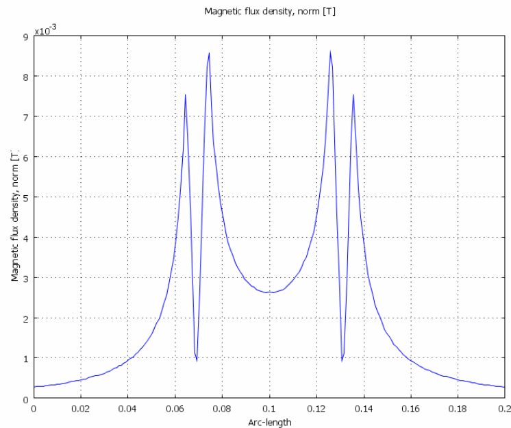
Figure 6.21 – Vertical cross-section plot of the magnetic flux density of two cables placed with a distance of 0.05 m between them.
