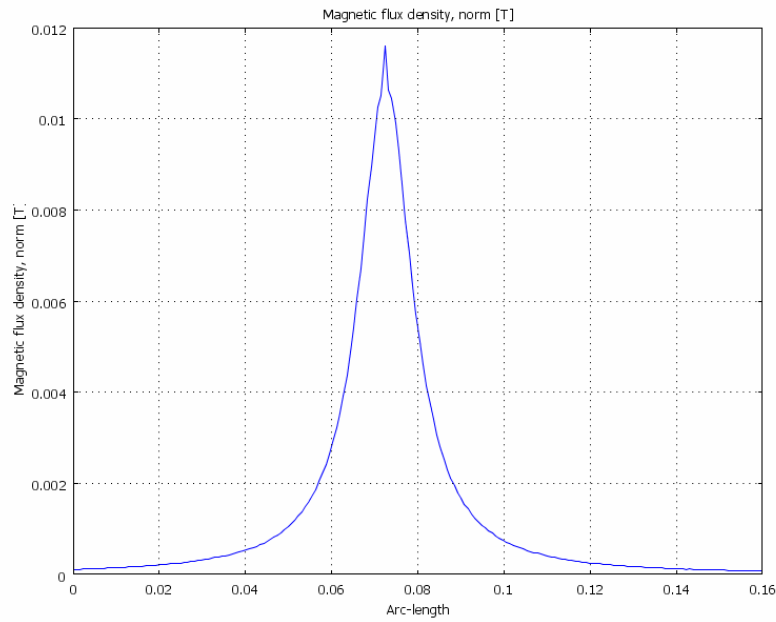
Figure 6.29 - Horizontal cross-section plot of the magnetic flux density of two shielded cables placed with no distance between them.
