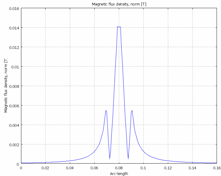
Figure 6.42 - Vertical cross-section plot of the magnetic flux density for a cable with two conductors with a common shield and a distance of 0.5 m to the magnetic girder.
