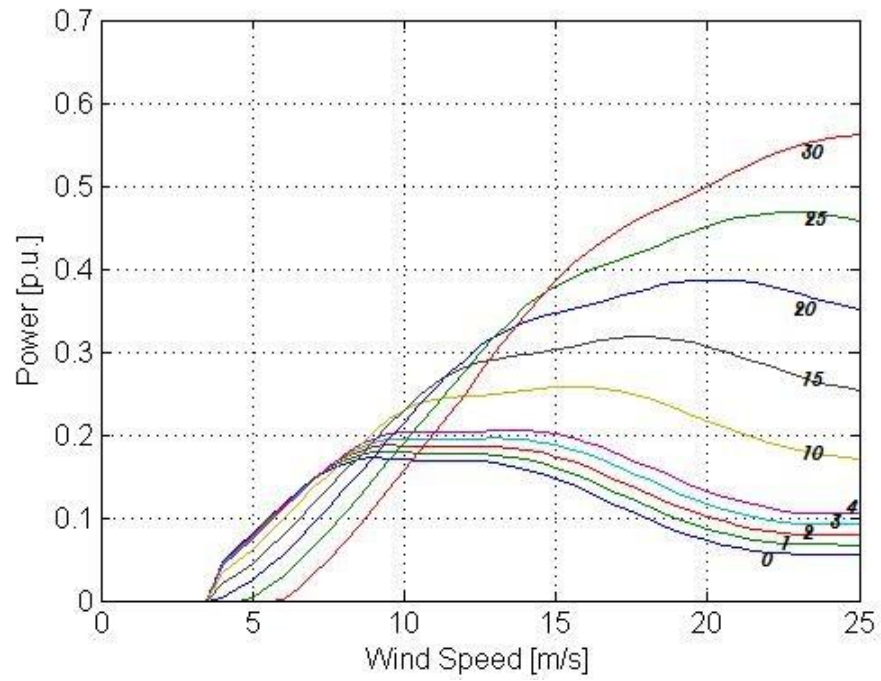
Figure 2.10: Output power vs. wind speed for different pitch angles at minimum rotor speed
