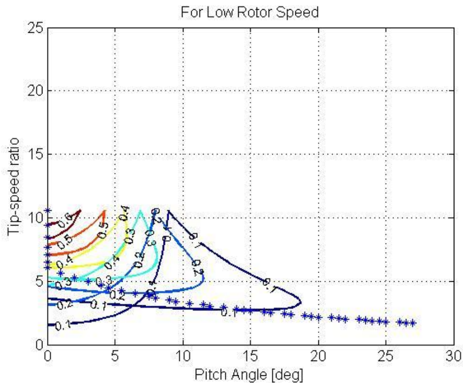
Figure 2.9: C_p(\lambda, \theta) expressed as contour lines where each lines shows a specific C_p value for minimum rotor speed. Starred line shows the optimal operation for different tip speed ratio and pitch angle combinations
