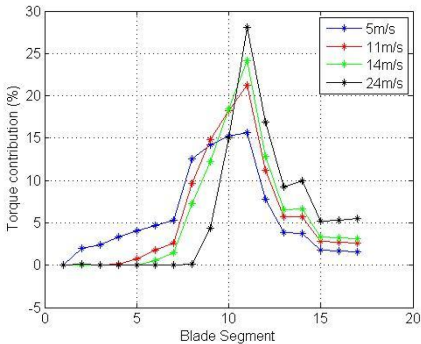
Figure 5.2: Torque contribution of each blade segment for different wind speeds
