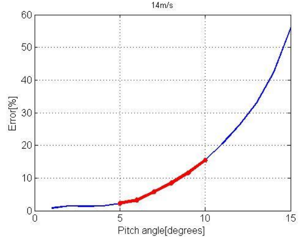
Figure 5.8: Error in torque output of original and analytical models for high wind speed range
