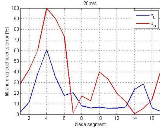
Figure 5.38: Lift and drag coefficients difference between the iterative and numerical calculations at each blade segment
