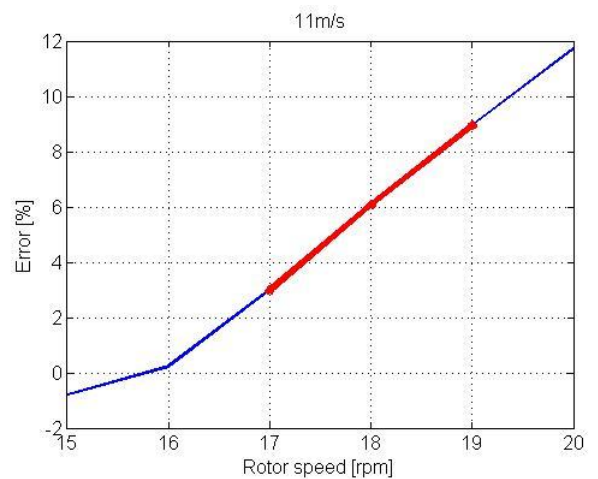
Figure 5.14: Error in torque output of original and analytical models for low wind speed range
