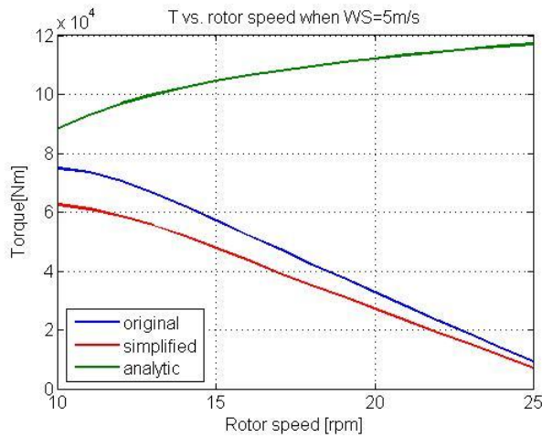
Figure 5.11: Torque vs. rotor speed at 5 m/s wind speed for original, simplified and analytical models
