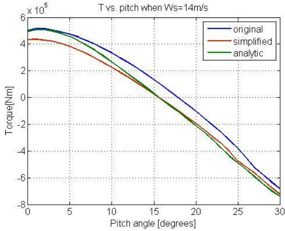
Figure 5.7: Torque vs. pitch angle at 14 m/s wind speed for original, simplified and analytical models
