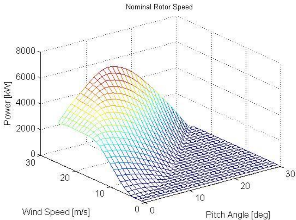
Figure 2.6: Power vs. wind speed and pitch angle for nominal rotor speed
