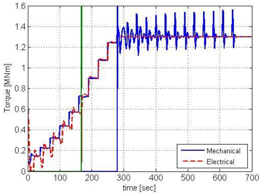
Figure 4.4: Torque response for whole speed range operation
