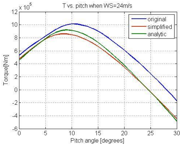
Figure 5.9: Torque vs. pitch angle at 24 m/s wind speed for original, simplified and analytical models
