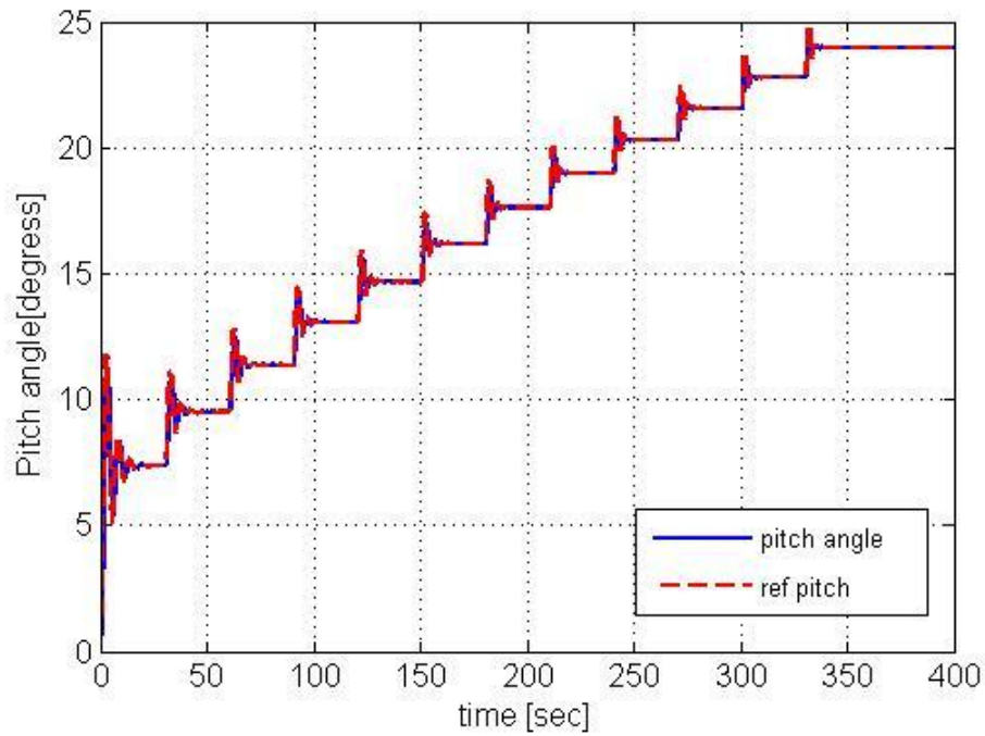
Figure 3.14: Pitch angle response for high wind speed region
