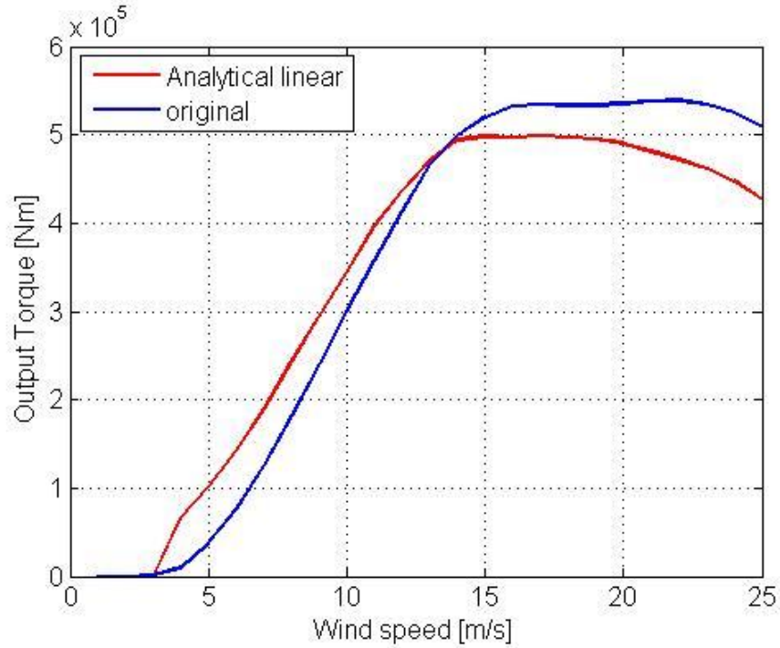
Figure 5.20: Torque vs. wind speed for different wind turbine models for middle speed operation
