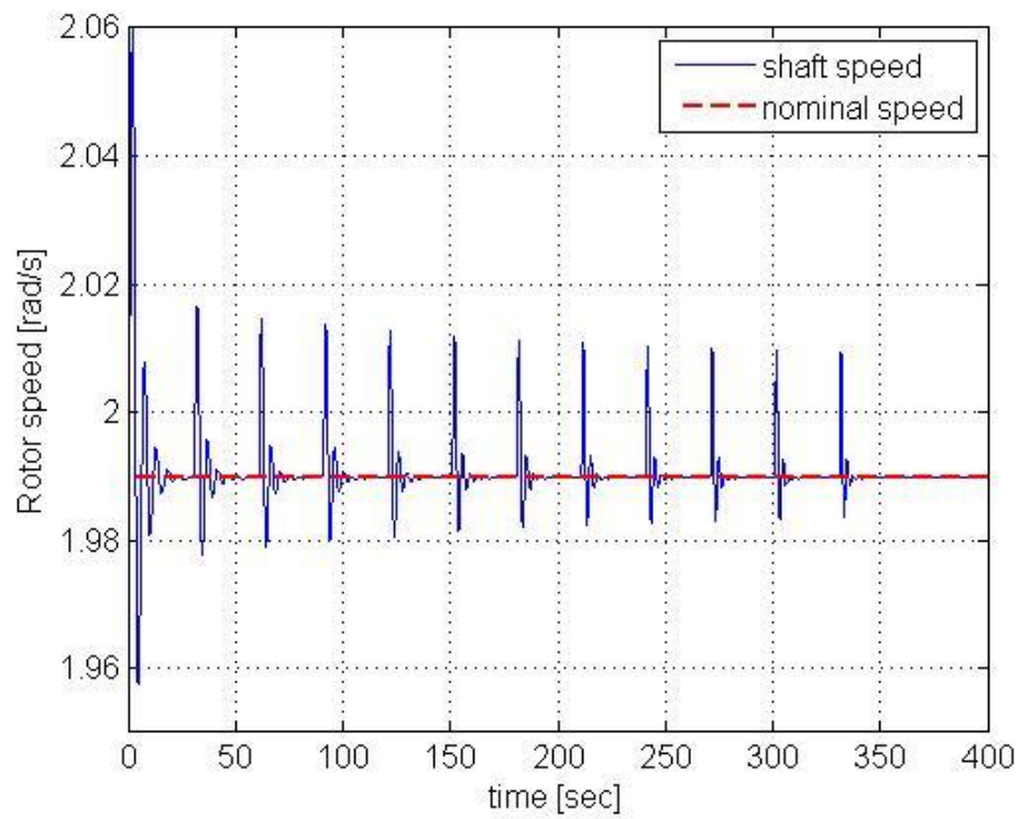
Figure 3.12: Rotor speed response for high wind speed region
