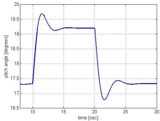
Figure 6.27: The pitch angle response during power down (25%)
