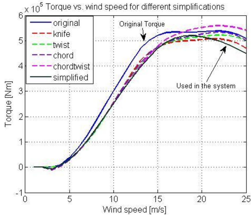
Figure 5.4: Torque vs. wind speed for different simplification adjustments
