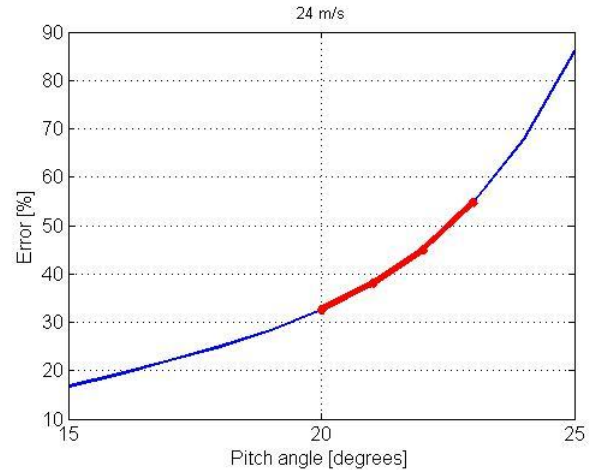
Figure 5.10: Error in torque output of original and analytical models for high wind speed range
