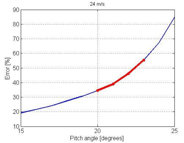
Figure 5.24: Error in torque output of original and analytical models for 24 m/s wind speed
