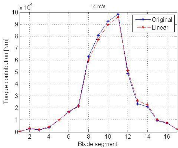
Figure 5.18: Torque contribution of each blade segment for original and linear aerodynamic data at 14m/s wind speed
