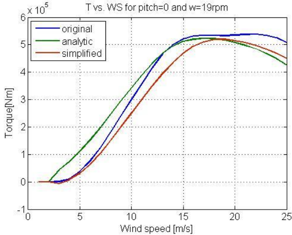
Figure 5.5: Torque vs. wind speed for original, simplified and analytical models
