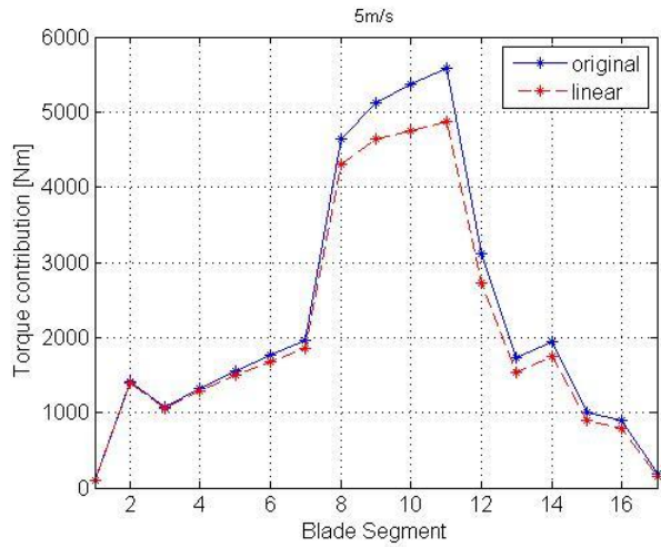
Figure 5.16: Torque contribution of each blade segment for original and linear aerodynamic data at 5m/s wind speed
