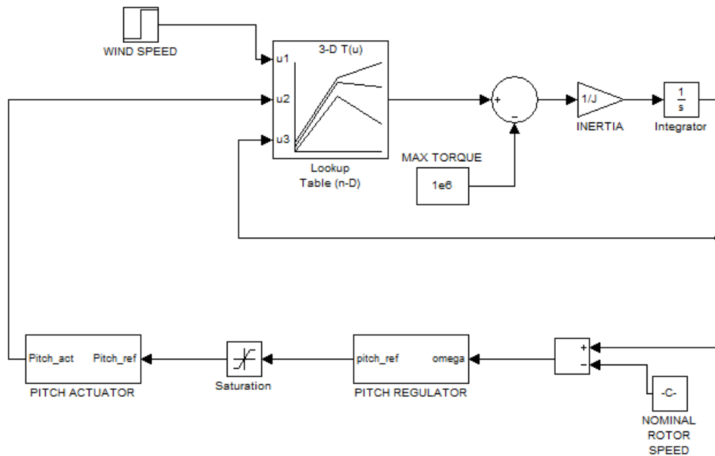
Figure 3.10: Control system for high speed interval
