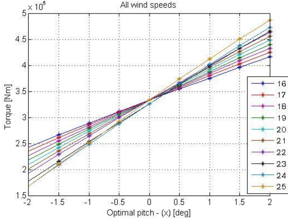
Figure 6.2: Output torque derivation according to small pitch angle changes for high wind speed region
