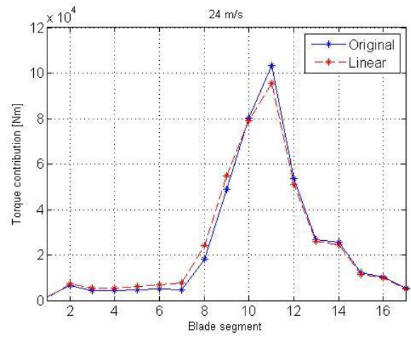
Figure 5.19: Torque contribution of each blade segment for original and linear aerodynamic data at 24m/s wind speed
