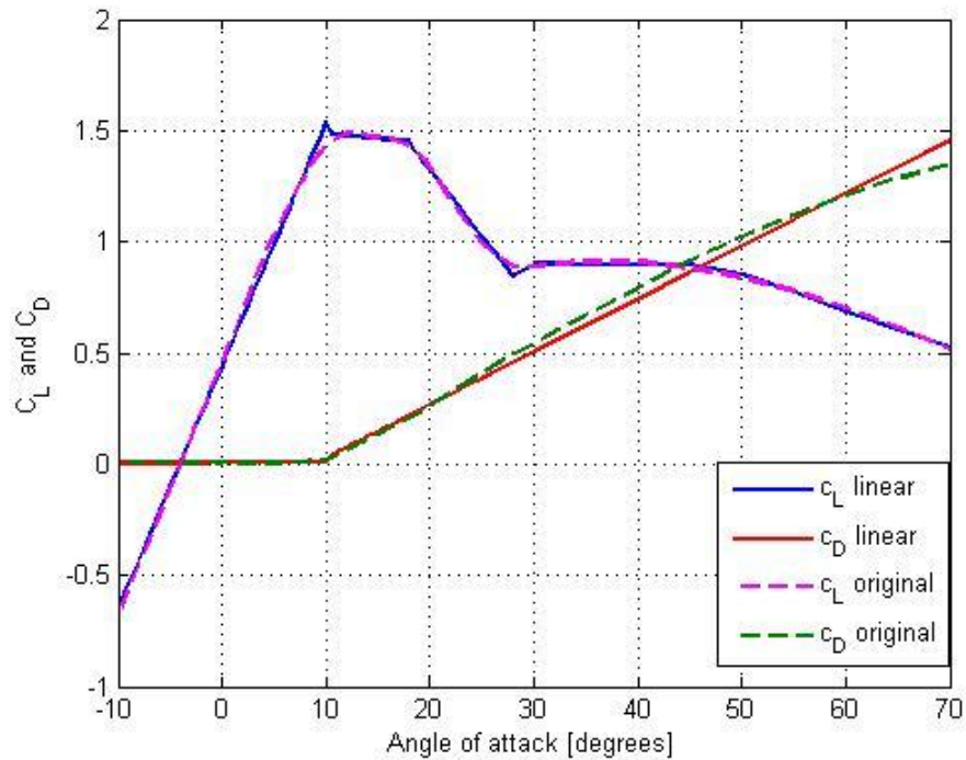
Figure 5.15: Linear fit of the lift and drag coefficient
