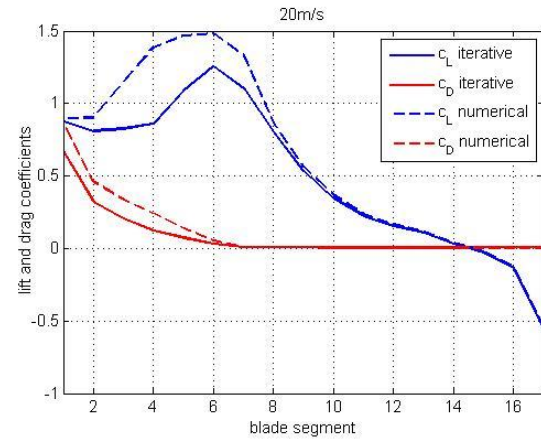
Figure 5.34: Lift and drag coefficients of each blade segment calculated by iterative and numerical methods
