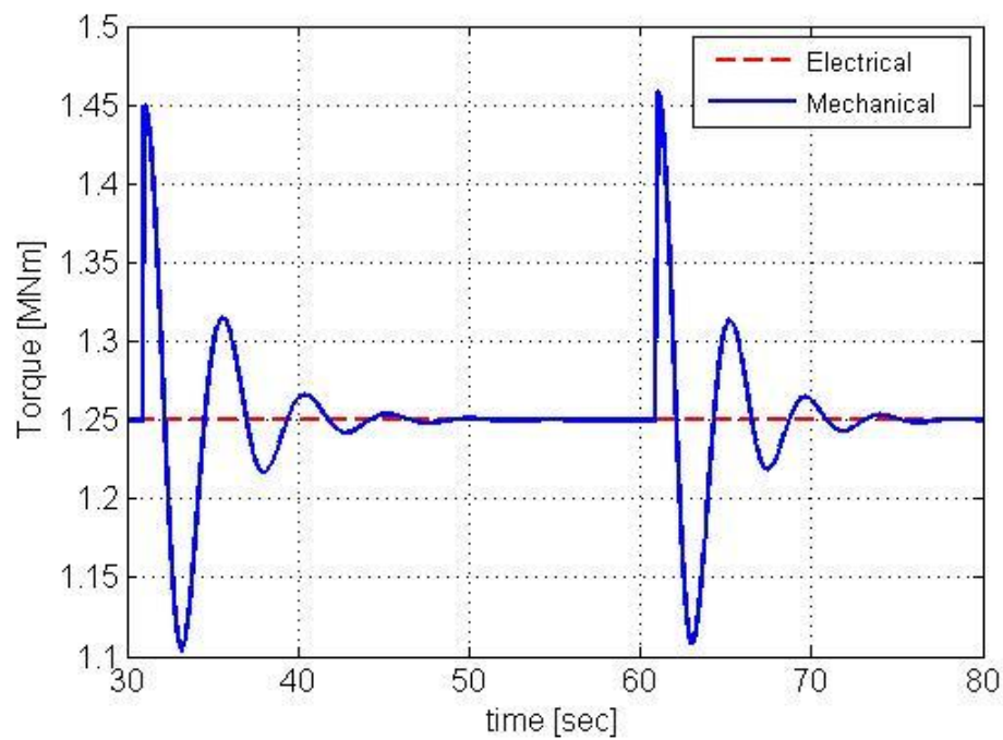
Figure 3.16: Details of torque response for high wind speed region
