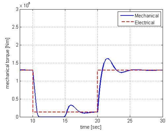
Figure 6.29: The output torque respond during power down (90%)
