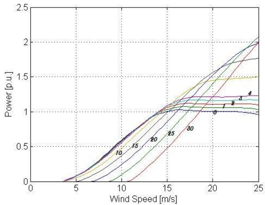
Figure 2.4: Output power vs. wind speed for different pitch angles for nominal rotor speed
