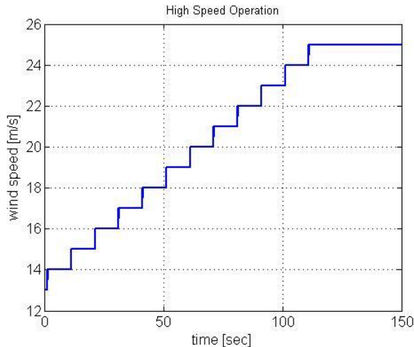
Figure 3.11 Wind speed response for high wind speed region
