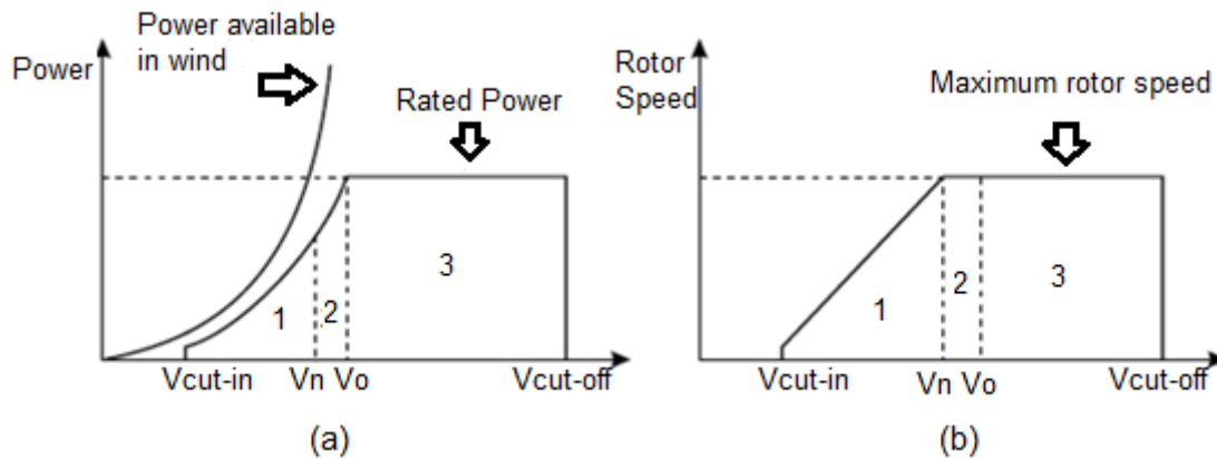
Figure 3.1: : (a) Output power for different wind speed ranges, (b) Rotor speed for different wind speed ranges from controller point of view
