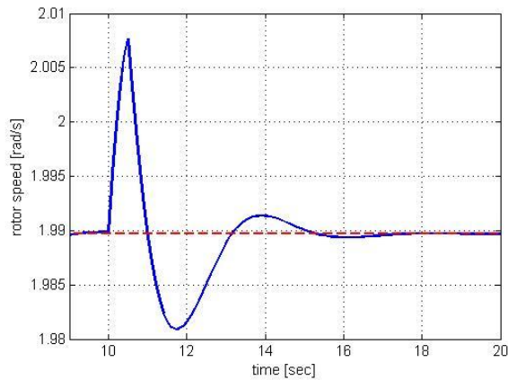
Figure 6.18: The rotor speed response (25% dip)
