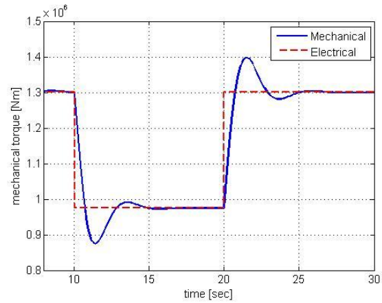
Figure 6.25: The output torque respond during power down (25%)
