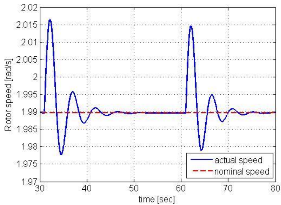
Figure 3.15: Details of rotor speed response for high wind speed region
