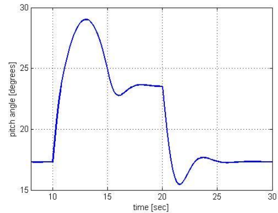
Figure 6.31: The pitch angle response during power down (90%)
