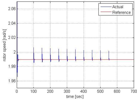
Figure 6.12: Rotor speed response of the pitch regulated system
