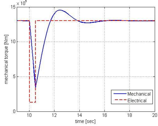
Figure 6.21: The output torque response (90% dip)
