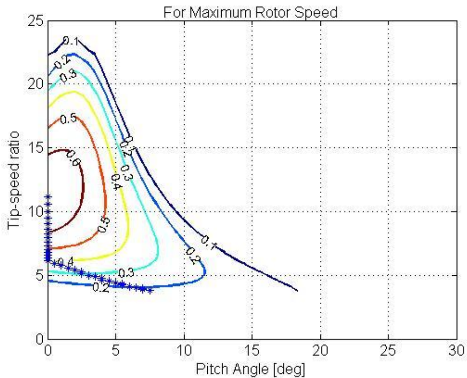
Figure 2.11: C_p(\lambda, \beta) expressed as contour lines where each line shows a specific C_p value for maximum rotor speed. Starred line shows the optimal operation for different tip speed ratio and pitch angle combinations
