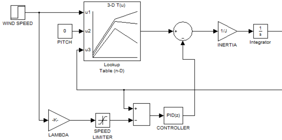
Figure 3.2: Control system for low speed interval
