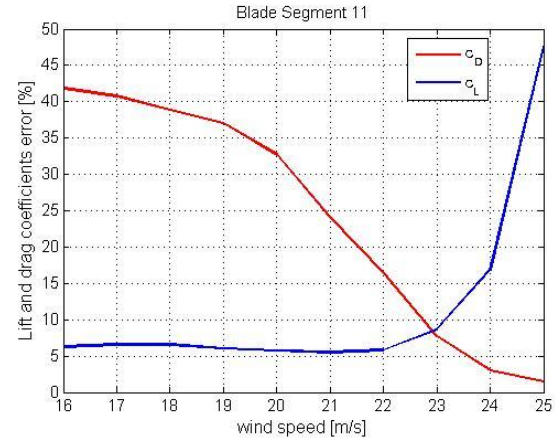
Figure 5.30: Lift and drag coefficients difference between the iterative and numerical calculations at 11 th blade segment
