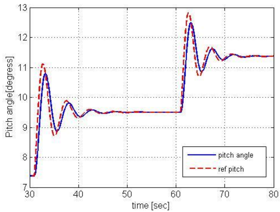
Figure 3.17: Details of pitch angle response for high wind speed region
