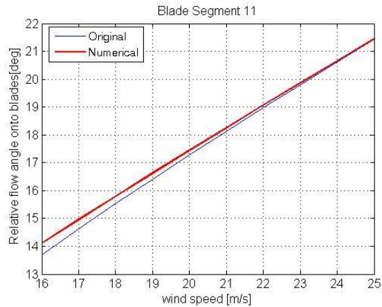
Figure 5.28: Relative flow angles onto blades obtained for the iterative and numerical BEM
