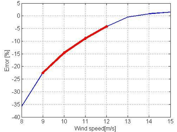
Figure 5.6: Error in torque output of original and analytical models for middle wind speed range
