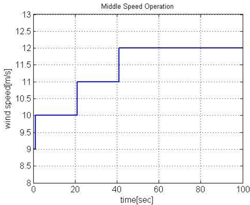
Figure 3.7: Wind speed response for middle wind speed region
