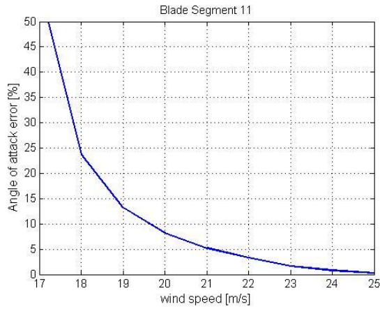
Figure 5.31: Angle of attack difference between the iterative and numerical calculations at 11 th blade segment
