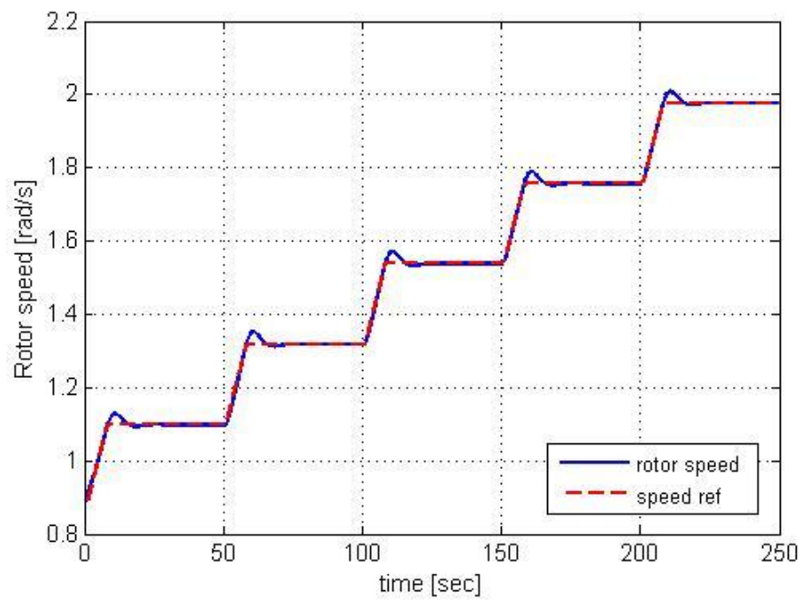
Figure 3.4: Rotor speed response for low wind speed region
