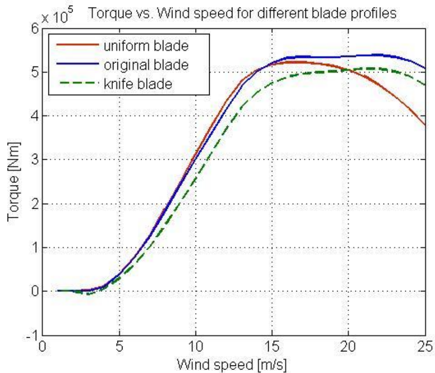
Figure 5.3: Torque vs. wind speed for different aerodynamic profiles
