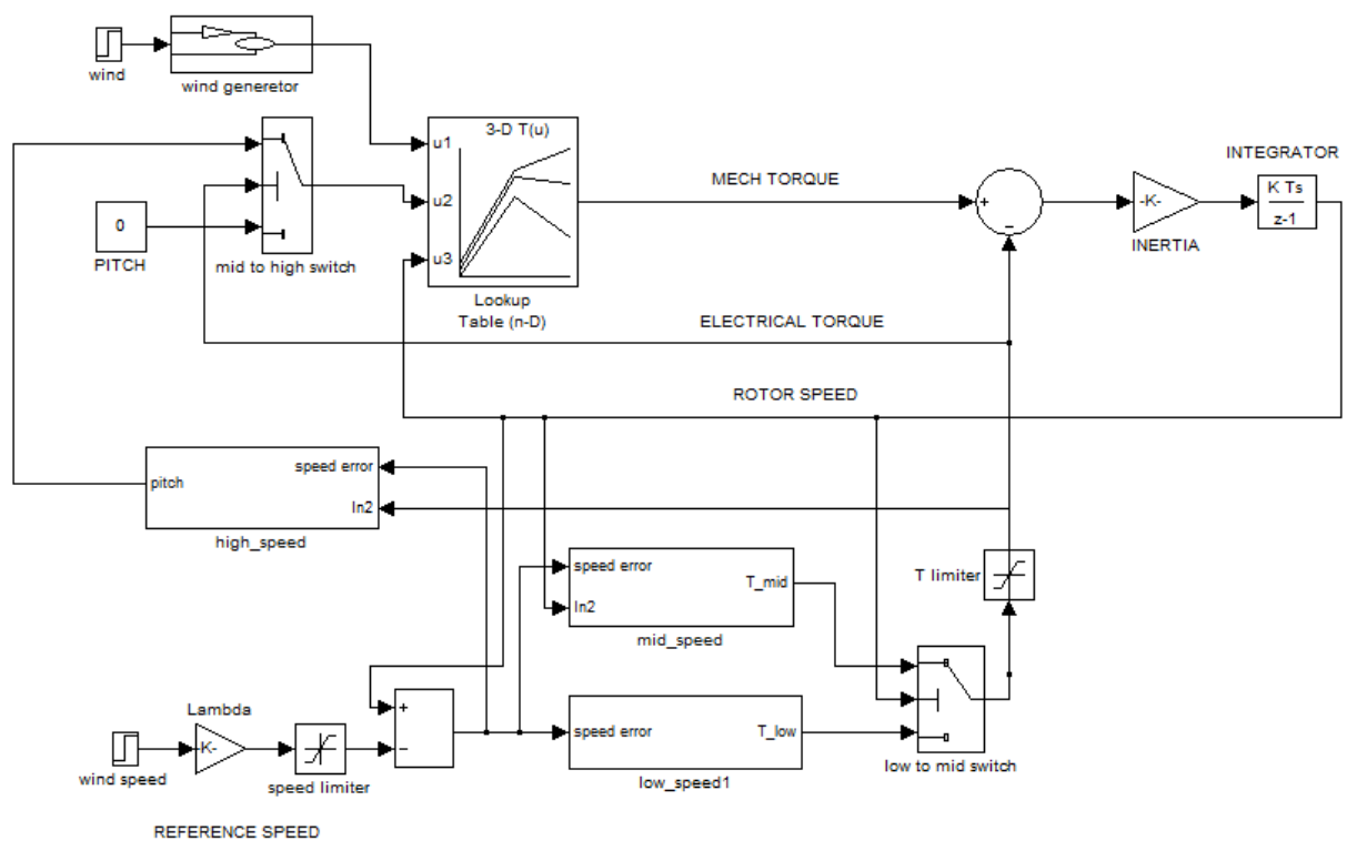
Figure 4.1: Control system for the whole wind speed range
