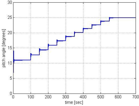
Figure 6.8: Pitch angle response of the pitch regulated system
