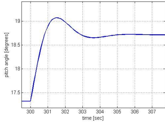
Figure 6.15: Pitch angle response of the pitch regulated system (close up)
