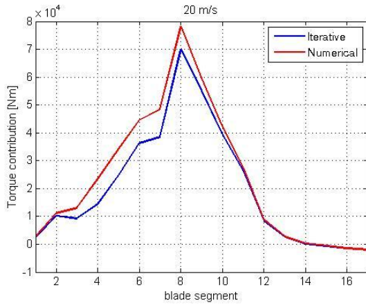
Figure 5.33: Torque contribution of each blade segment calculated by iterative and numerical methods
