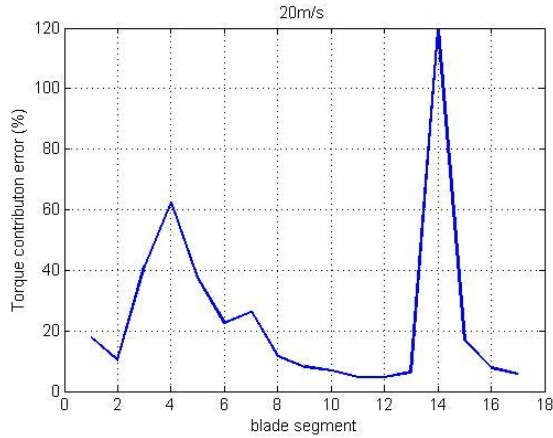
Figure 5.37: Torque difference between the iterative and numerical calculations at each blade segment
