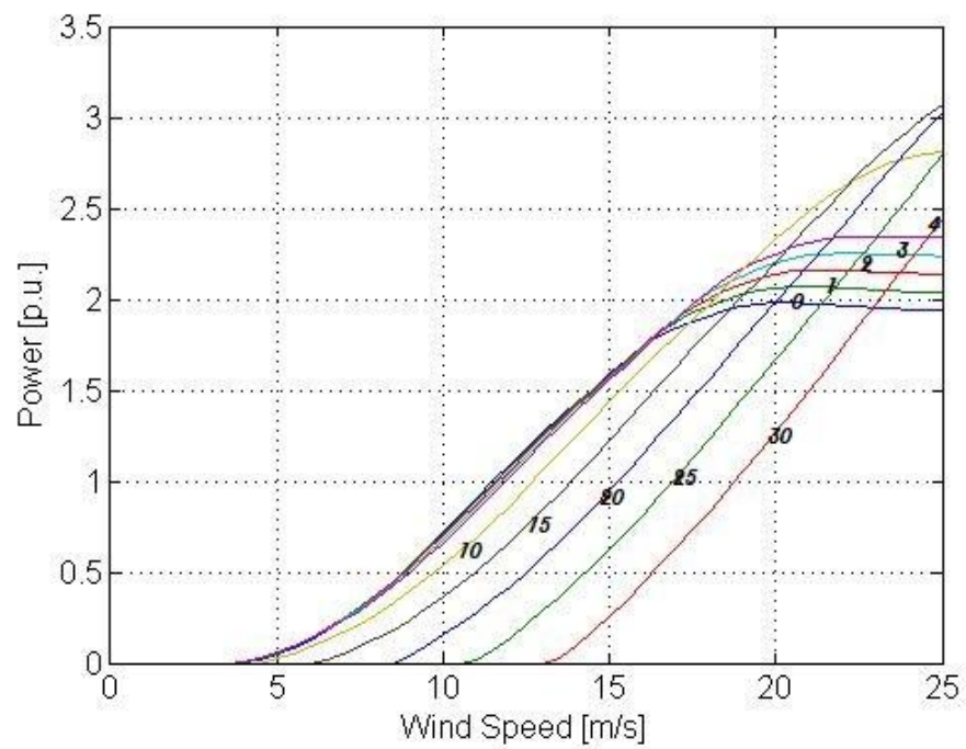
Figure 2.12: Output power vs. wind speed for different pitch angles at maximum rotor speed
