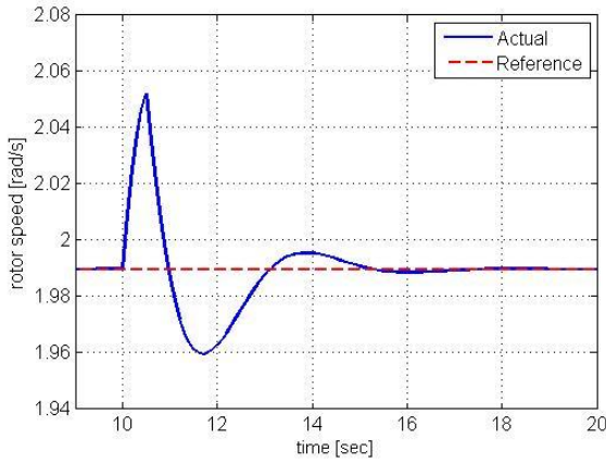
Figure 6.22: The rotor speed response (90% dip)
