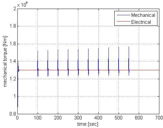
Figure 6.4: Mechanical and electrical torque response of the pitch regulated system
