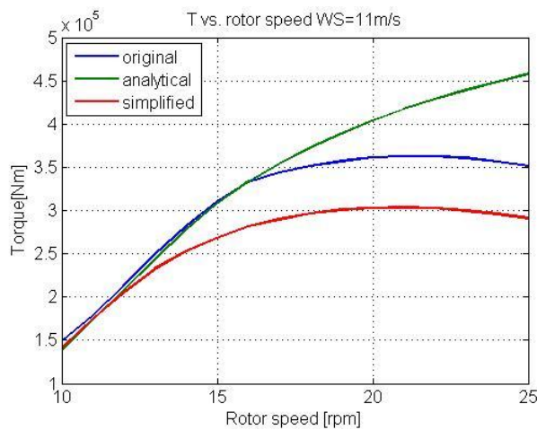
Figure 5.13: Torque vs. rotor speed at 11 m/s wind speed for original, simplified and analytical models
