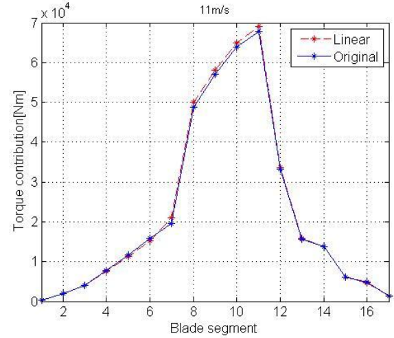
Figure 5.17: Torque contribution of each blade segment for original and linear aerodynamic data at 11m/s wind speed
