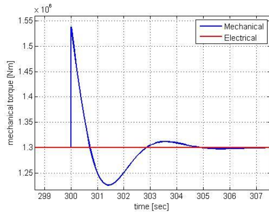
Figure 6.11: Mechanical and electrical torque response of the pitch regulated system (close up)
