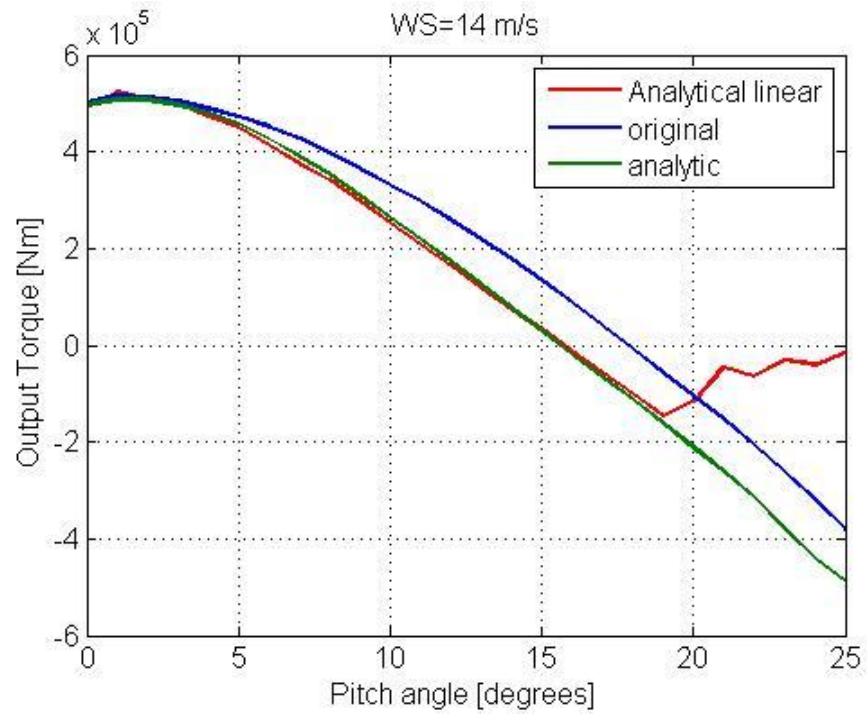
Figure 5.21: Torque vs. pitch angle at 14 m/s wind speed for original, analytic and linear analytical models
