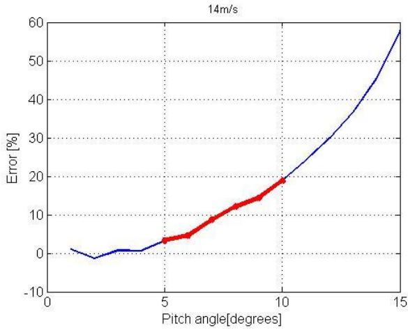
Figure 5.23: Error in torque output of original and analytical models for 14 m/s wind speed
