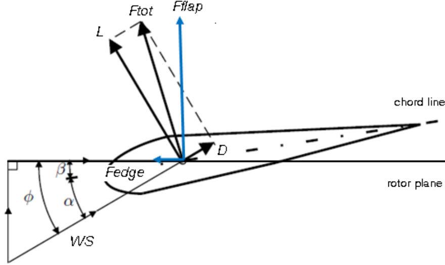
Figure 2.3: Wind and forces on the rotor plane
