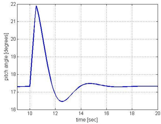
Figure 6.23: The pitch angle response (90% dip)
