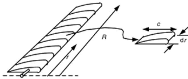
Figure 5.1: Schematic of the blade elements
