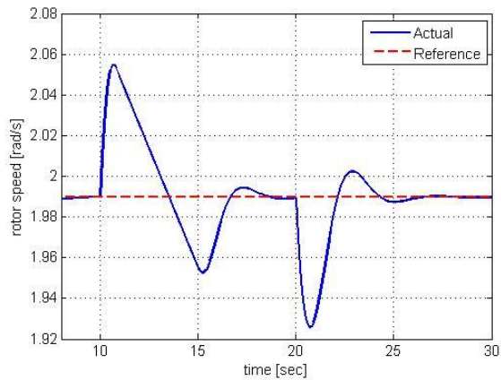
Figure 6.30: The rotor speed response during power down (90%)
