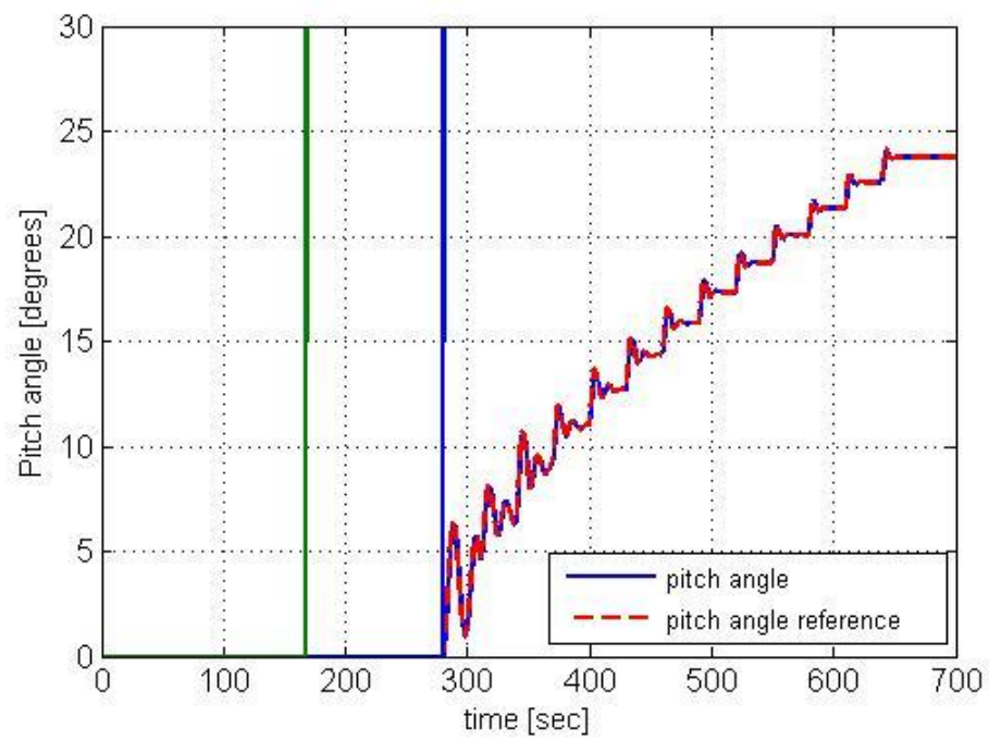
Figure 4.5: Pitch angle response for whole speed range operation
