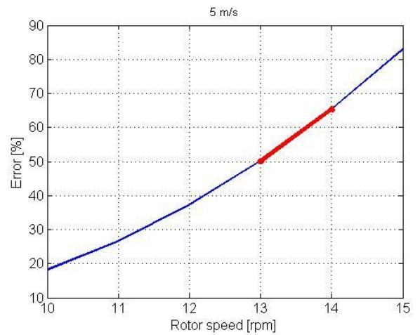
Figure 5.12: Error in torque output of original and analytical models for low wind speed range
