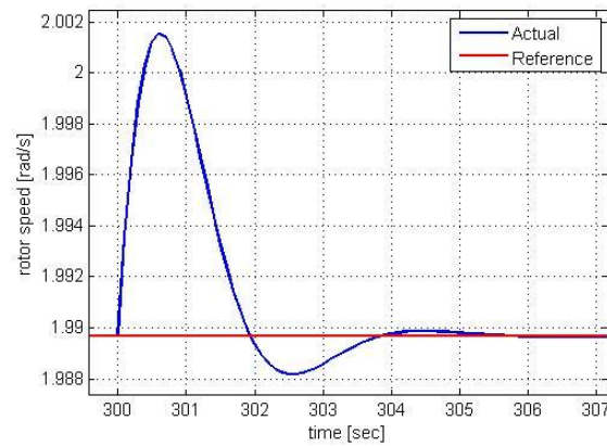
Figure 6.7: Rotor speed response of the pitch regulated system (close up)
