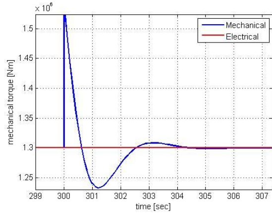
Figure 6.5: Mechanical and electrical torque response of the pitch regulated system (close up)
