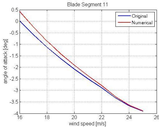
Figure 5.27: Angle of attack obtained for the iterative and numerical BEM
