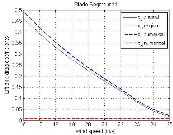
Figure 5.26: Lift and drag coefficients obtained for the iterative and numerical BEM
