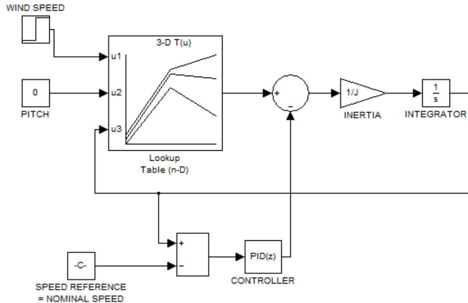
Figure 3.6: Control system for middle speed interval
