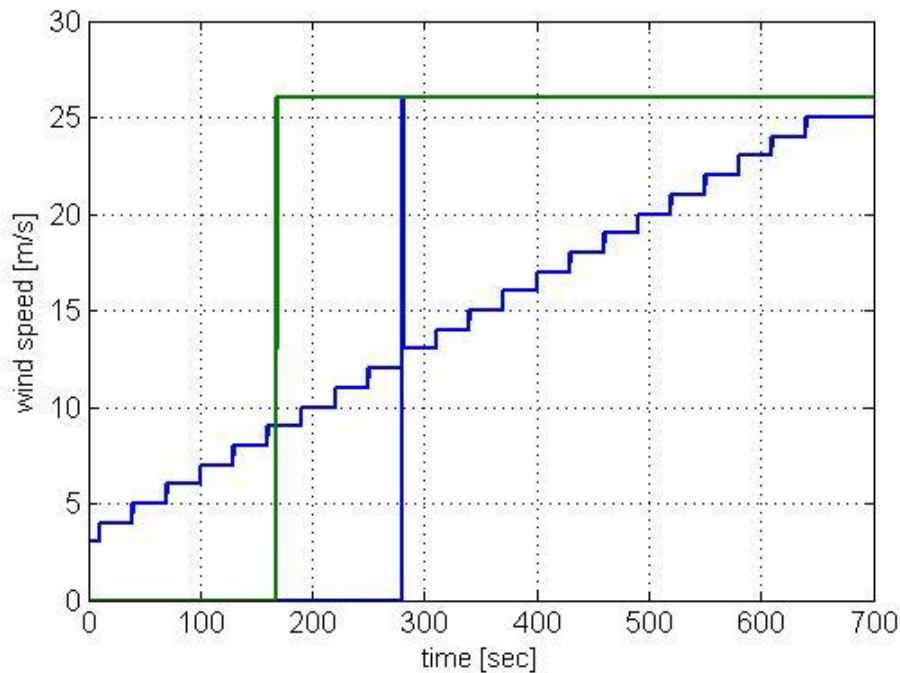
Figure 4.2: Wind speed steps for whole speed range operation
