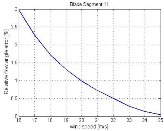
Figure 5.32: Relative flow angle difference between the iterative and numerical calculations at 11 th blade segment
