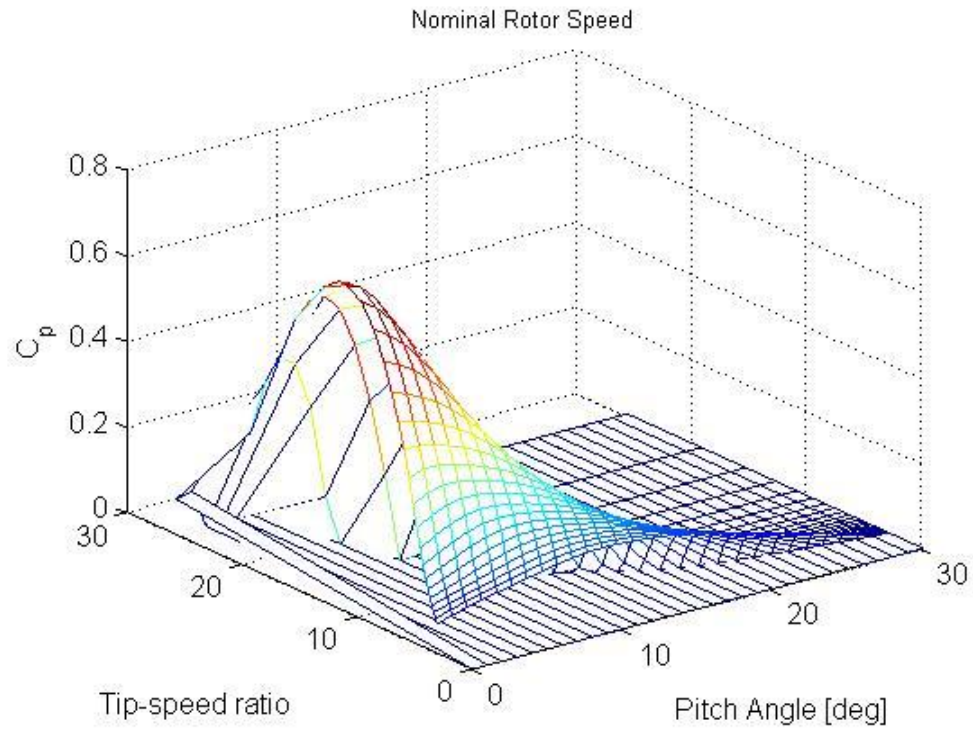
Figure 2.7: C_p(\lambda, \beta) for nominal rotor speed
