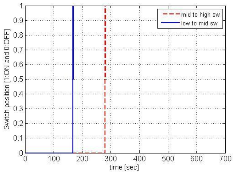
Figure 4.6: Switching pattern for the whole speed range operation
