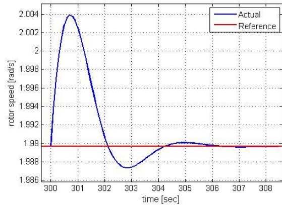
Figure 6.13: Rotor speed response of the pitch regulated system (close up)
