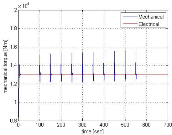
Figure 6.10: Mechanical and electrical torque response of the pitch regulated system
