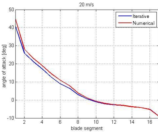
Figure 5.35: Angle of attack of each blade segment calculated by iterative and numerical methods
