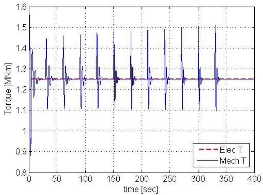
Figure 3.13: Torque response for high wind speed region
