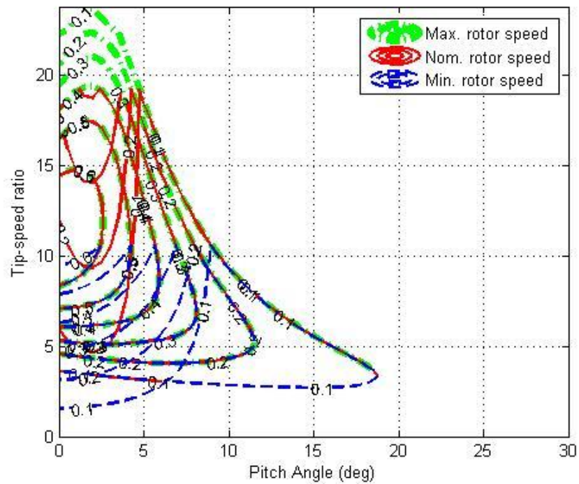
Figure 2.13: Comparison of the C_p values for different rotor speed levels
