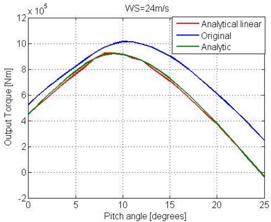
Figure 5.22: Torque vs. pitch angle at 24 m/s wind speed for original, analytic and linear analytical models
