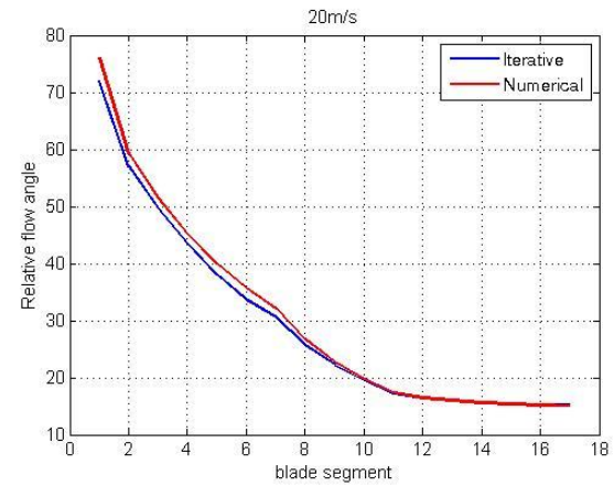
Figure 5.36: Relative flow angle of each blade segment calculated by iterative and numerical methods
