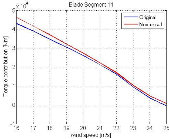
Figure 5.25: Torque produced by 11 th blade segment for the iterative and numerical BEM
