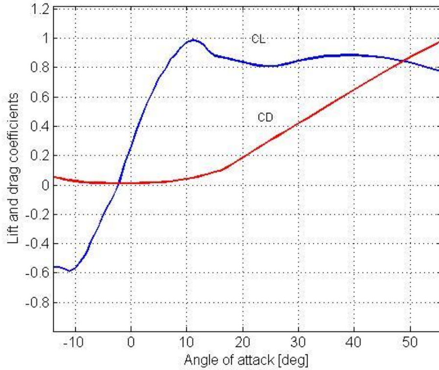
Figure 2.2: Lift and drag coefficients of the airfoil according to the angle of attack
