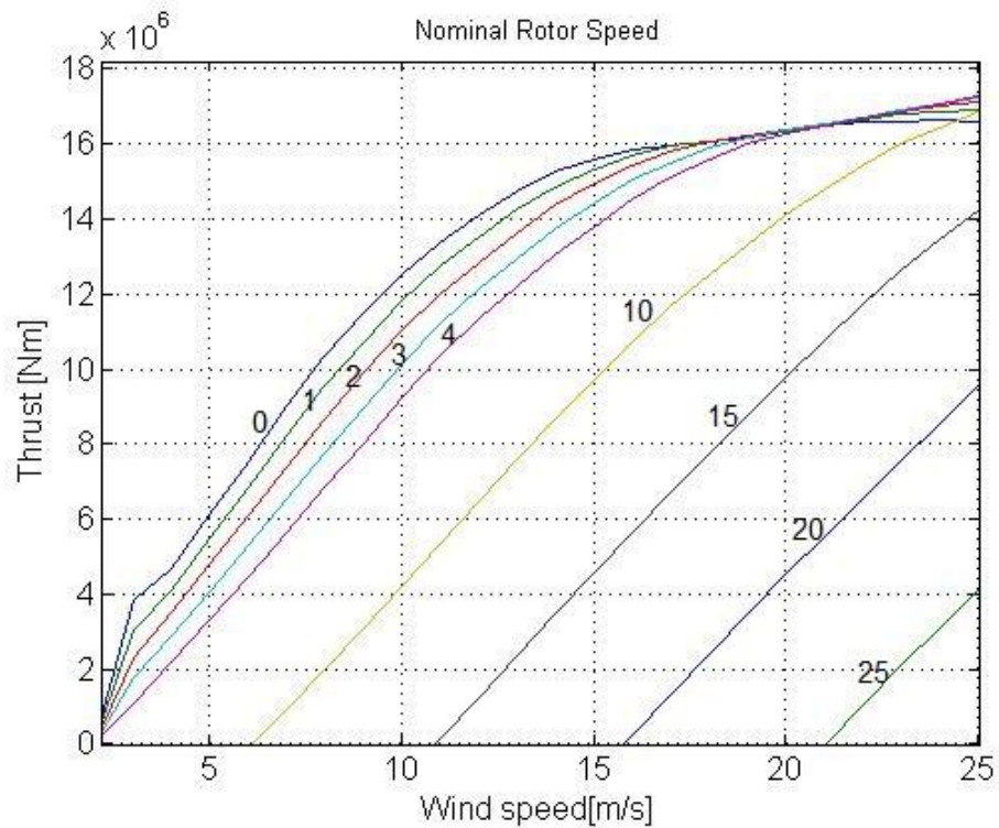
Figure 2.5: Power from the thrust vs. wind speed for different pitch angles
