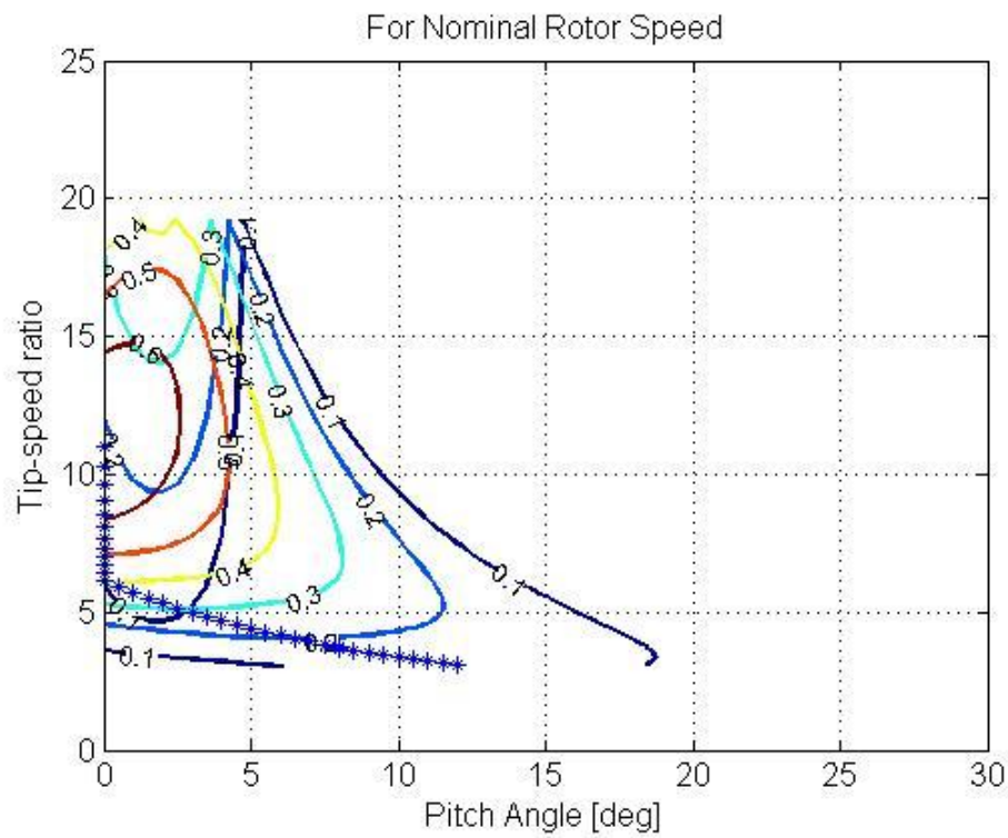
Figure 2.8: C_p(\lambda, \beta) expressed as contour lines where each lines shows a specific C_p value for nominal rotor speed. Starred line shows the optimal operation for different tip speed ratio and pitch angle combinations
