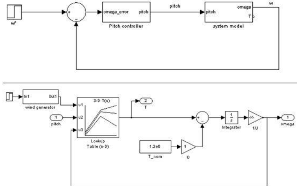
Figure 6.3: Scheme of the pitch regulated high speed control and the wind turbine system model
