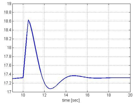
Figure 6.19: The pitch angle response (25% dip)
