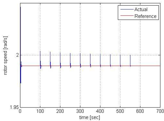
Figure 6.6: Rotor speed response of the pitch regulated system
