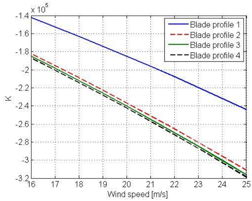
Figure C.1: Comparison of the K values obtained by using different blade profiles
