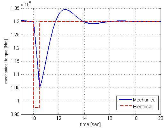
Figure 6.17: The output torque response (25% dip)
