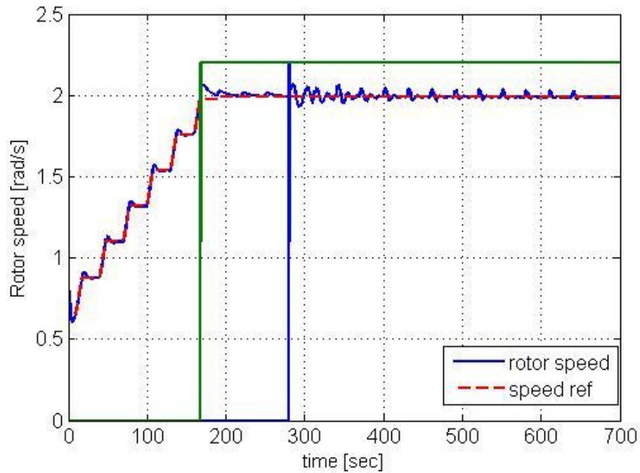
Figure 4.3: Rotor speed response for whole speed range operation
