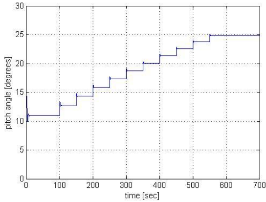
Figure 6.14: Pitch angle response of the pitch regulated system
