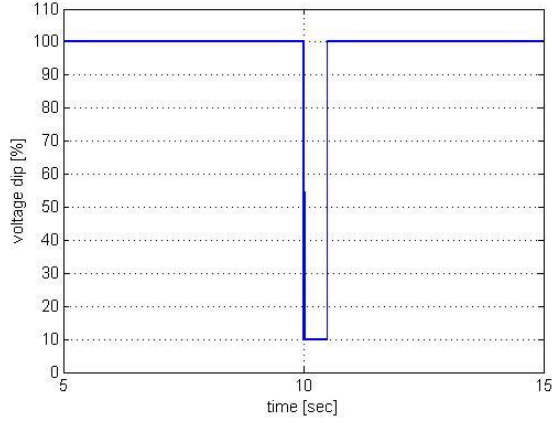
Figure 6.20: The grid voltage (90% dip)
