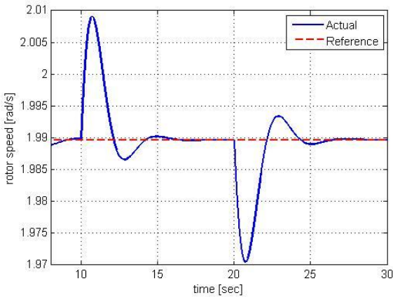
Figure 6.26: The rotor speed response during power down (25%)
