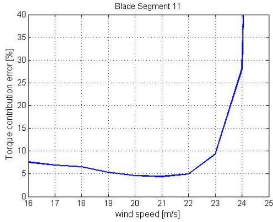
Figure 5.29: Torque difference between the iterative and numerical calculations at 11 th blade segment
