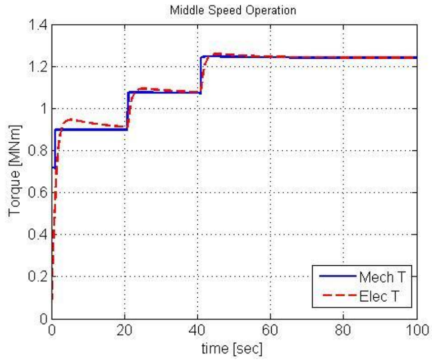
Figure 3.9: Torque response for middle wind speed region
