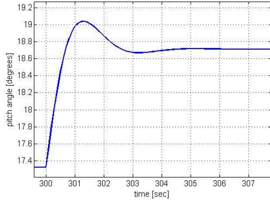
Figure 6.9: Pitch angle response of the pitch regulated system (close up)
