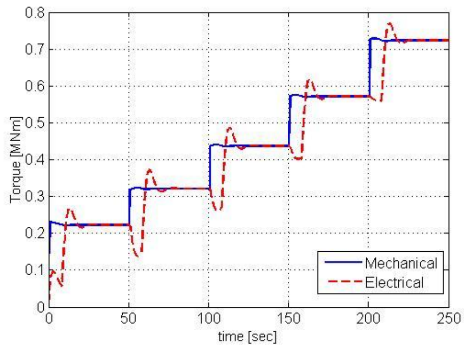
Figure 3.5: Torque response for low wind speed region
