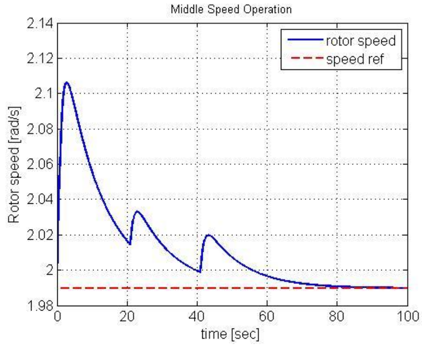
Figure 3.8: Rotor speed response for middle wind speed region
