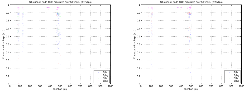
Figure 5.8: Scatter plot of dip situation. Original line setup (left) and shieldning added to all 130 kV lines (right).
