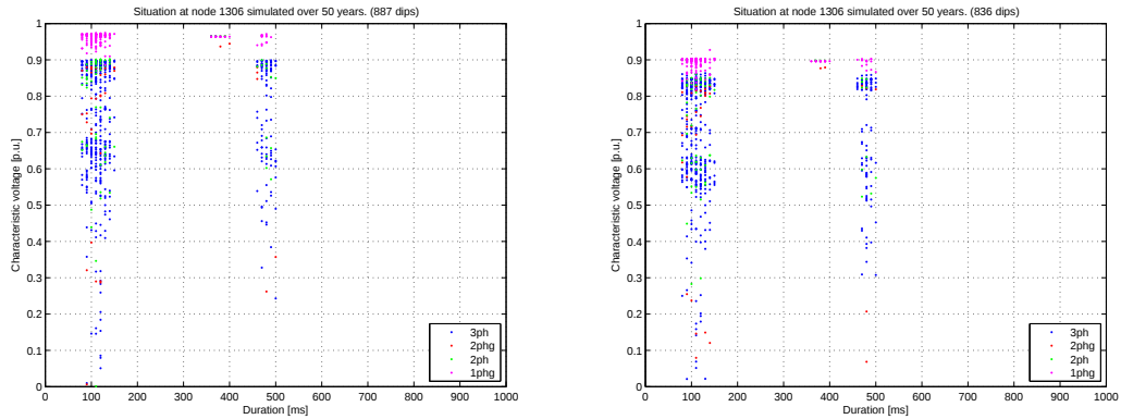
Figure 5.14: Scatter plot of dip situation. Original line setup (left) and with line disconnected (right).
