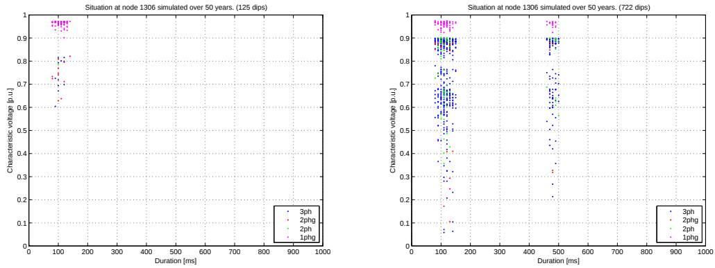
Figure 5.3: Only faults on 400 kV (left). Only faults on 130 kV (right).
