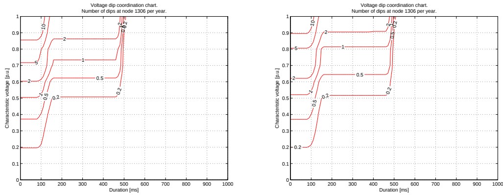
Figure 5.9: Coordination chart. Original line setup (left) and shieldning added to all 130 kV lines (right).
